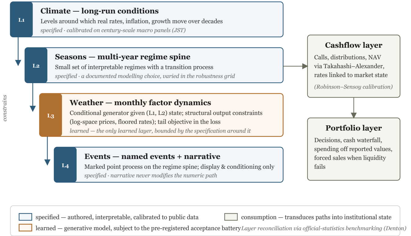
Figure 2 — Four generator layers from slow to fast, each constraining the next, with the two consumption layers. L3 is the only learned layer, bounded above and below by specification.
