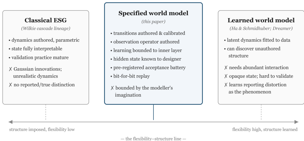
Figure 1 — The design point. Specified world models sit between classical economic scenario generators and learned world models on the flexibility–structure line, taking interpretable authored dynamics from the former and bounded generative flexibility from the latter.
