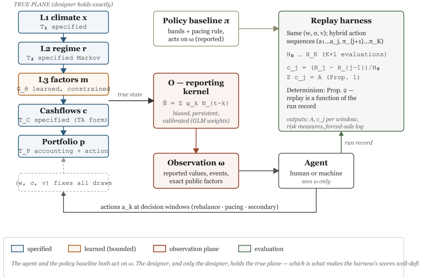
Figure 7 — The complete system: generator layers produce the true state, the observation operator produces the reported plane, the agent acts through decision windows, and the replay harness scores each decision against the policy baseline on the same fixed path.
