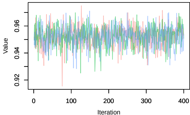
Trace – phi.age[2]
