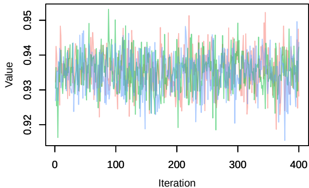
Trace – phi.age[5]
