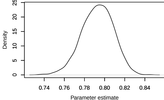
Density – phi.age[9]
