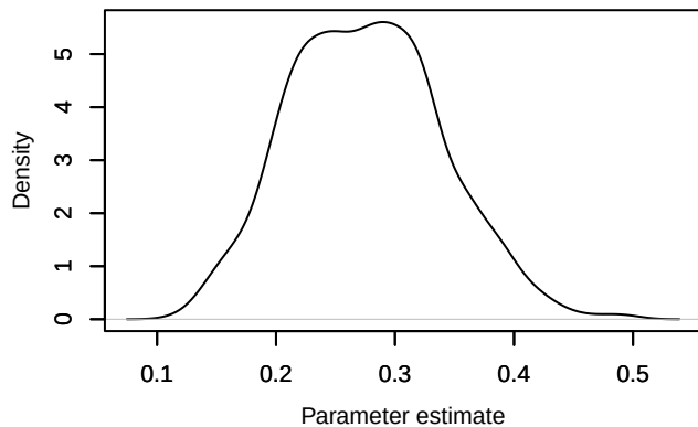
Density – phi.age[12]
