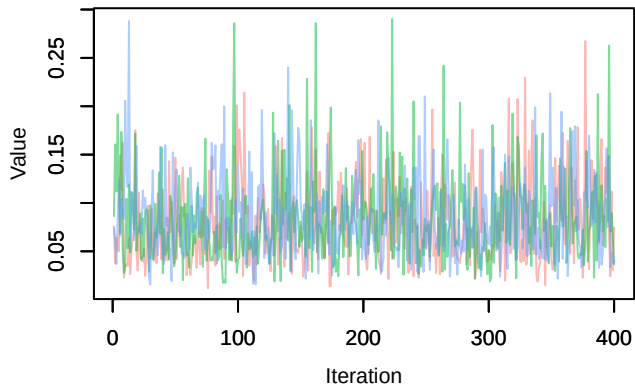
Trace – phi.age[15]
