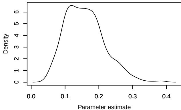
Density – phi.age[14]
