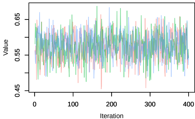
Trace – phi.age[11]
