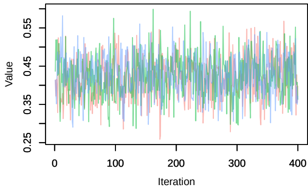
Trace – phi.age[12]
