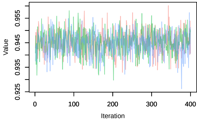
Trace – phi.age[3]
