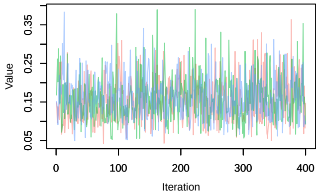
Trace – phi.age[14]
