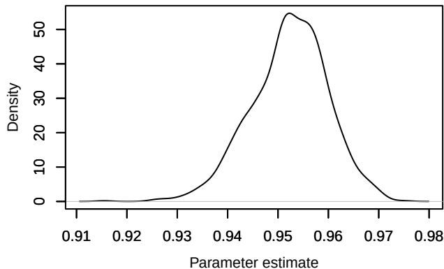
Density – phi.age[2]
