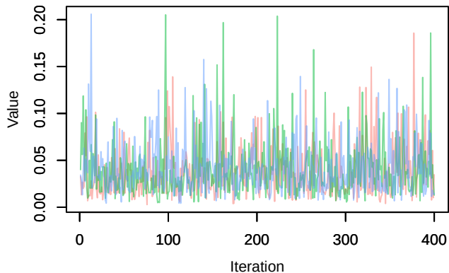
Trace – phi.age[15]
