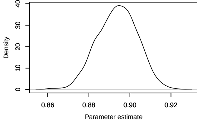
Density – phi.age[6]
