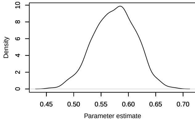
Density – phi.age[11]
