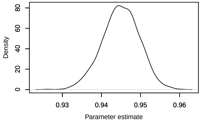
Density – phi.age[3]
