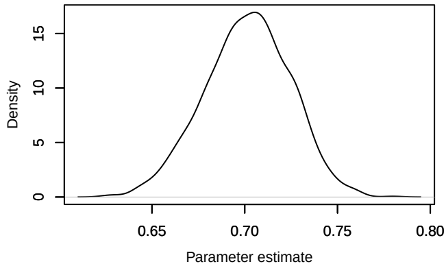
Density – phi.age[9]
