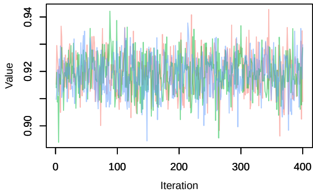
Trace – phi.age[6]
