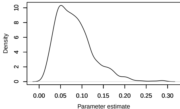
Density – phi.age[15]
