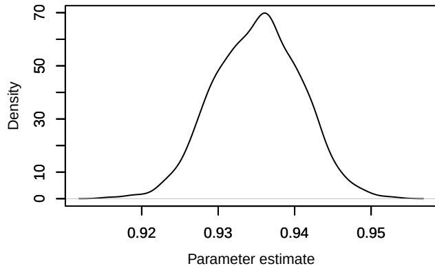
Density – phi.age[5]
