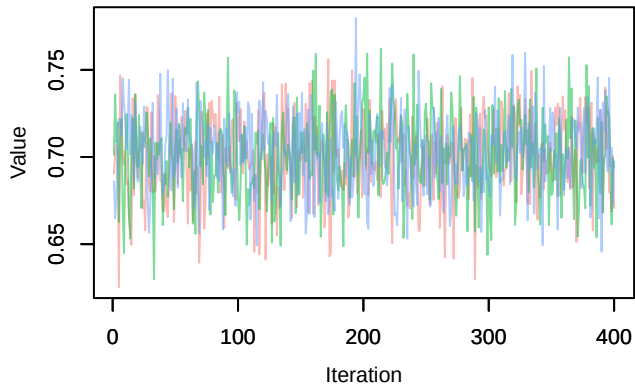
Trace – phi.age[9]
