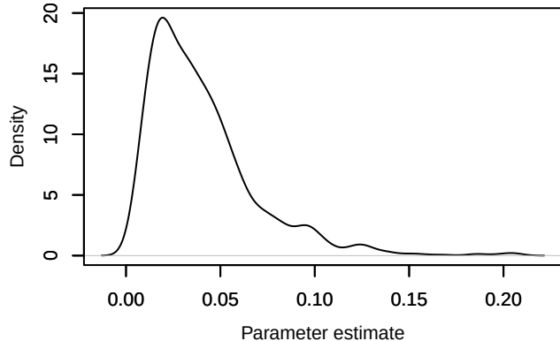
Density – phi.age[15]
