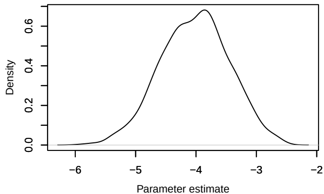
Density – beta1[11]
