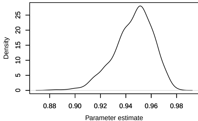
Density – phi.year[9]
