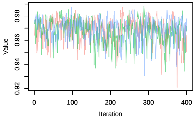
Trace – phi.year[6]
