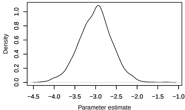
Density – beta1[11]
