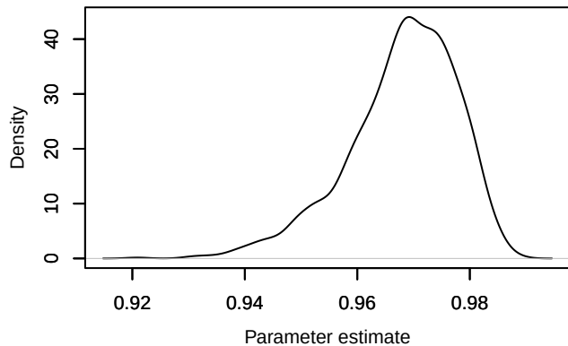
Density – phi.year[6]
