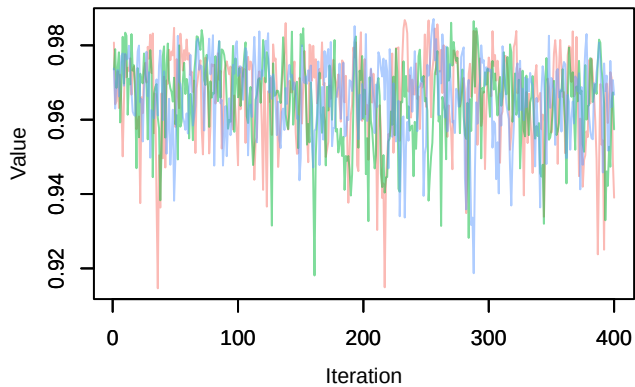
Trace – phi.year[4]
