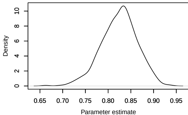
Density – phi.age[9]
