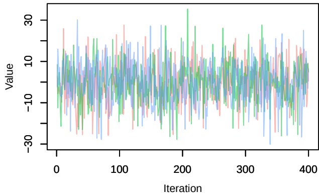
Trace – beta1[14]
