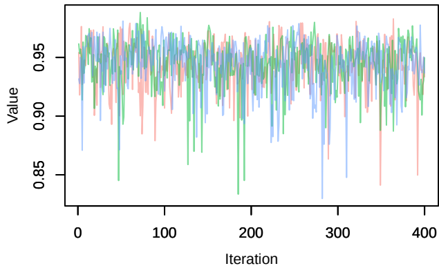
Trace – phi.year[13]
