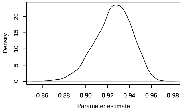
Density – phi.age[4]
