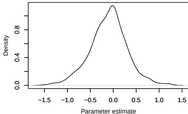
Density – phi.age[1]
