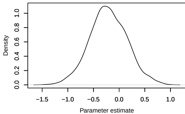
Density – beta1[5]
