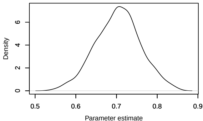
Density – phi.age[9]
