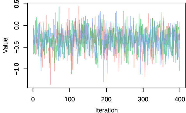
Trace – eps1[9]
