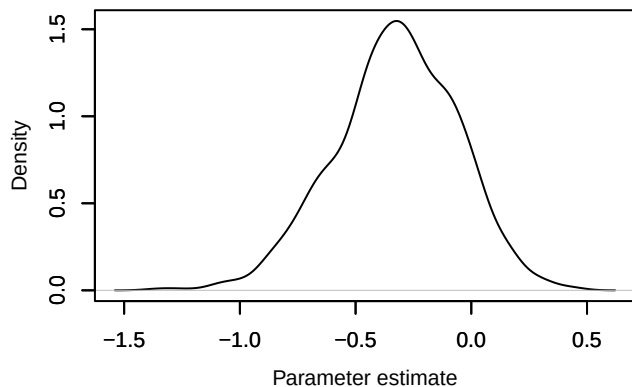
Density – eps1[9]
