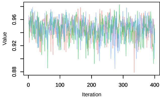
Trace – phi.year[9]
