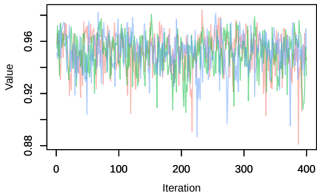
Trace – phi.year[3]
