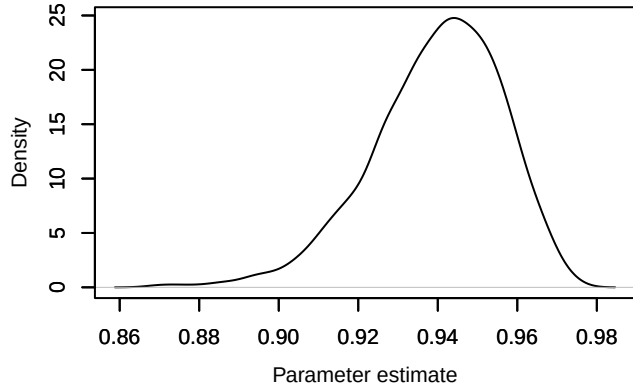
Density – phi.year[7]
