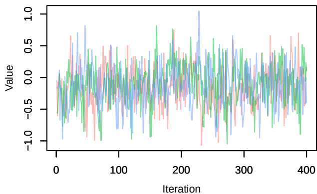
Trace – beta1[2]
