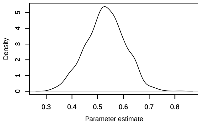
Density – phi.age[10]
