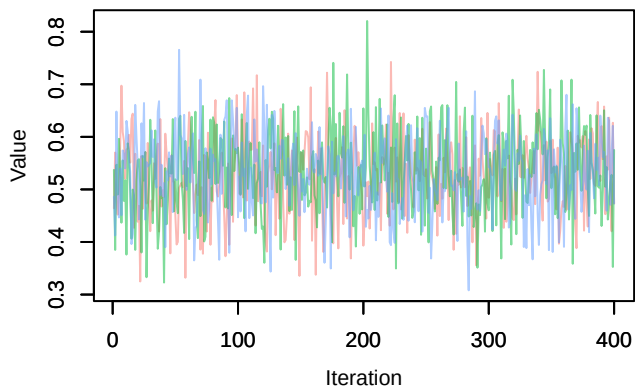
Trace – phi.age[10]
