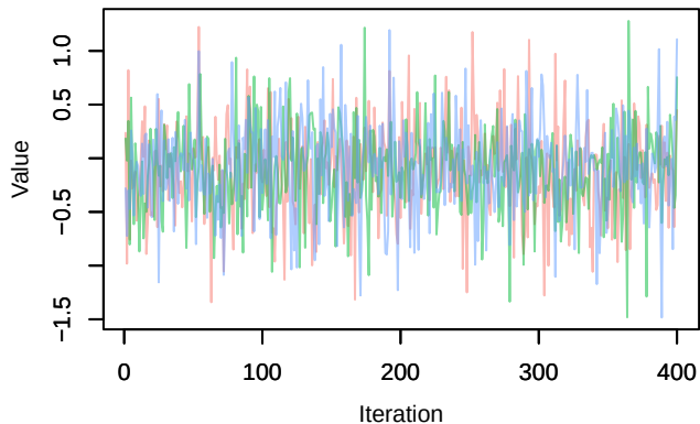
Trace – phi.age[1]
