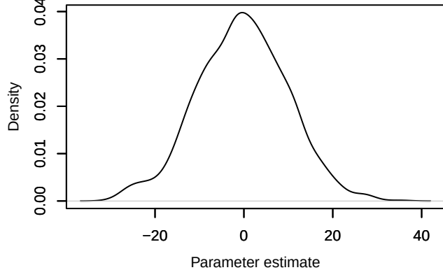
Density – beta1[14]
