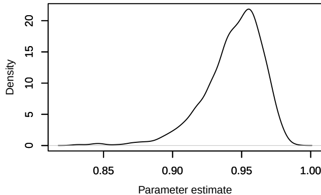
Density – phi.year[13]
