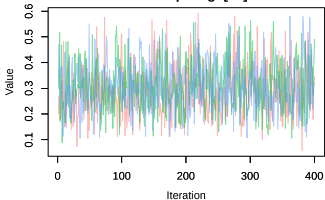
Trace – phi.age[12]
