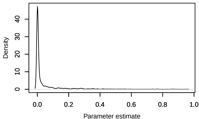
Density – phi.year[1]
