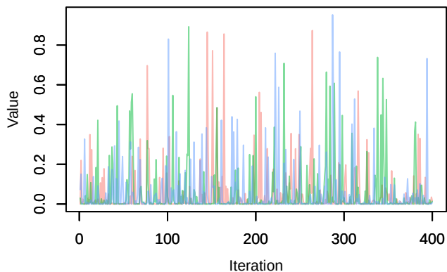
Trace – phi.year[1]
