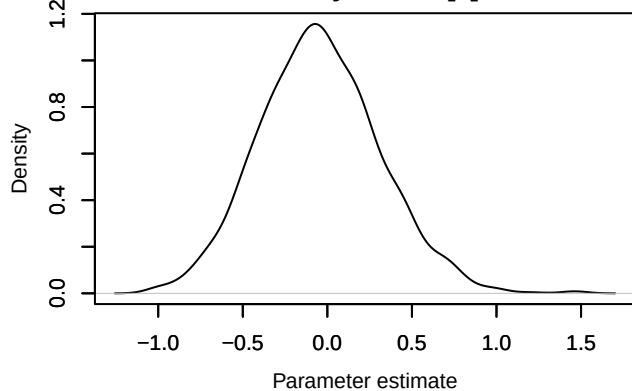
Density – beta1[4]
