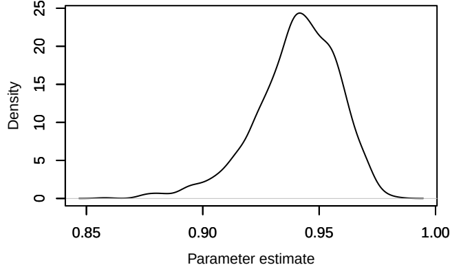
Density – phi.year[10]
