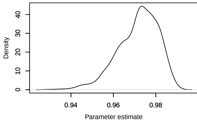
Density – phi.year[4]
