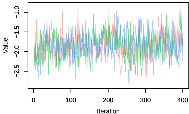
Trace – beta1[8]
