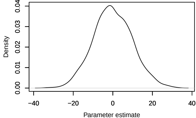
Density – beta1[14]
