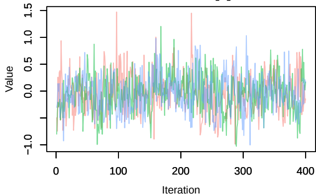
Trace – beta1[4]
