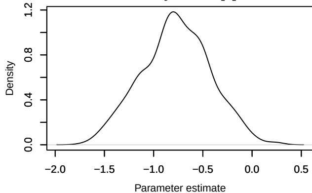
Density – beta1[7]
