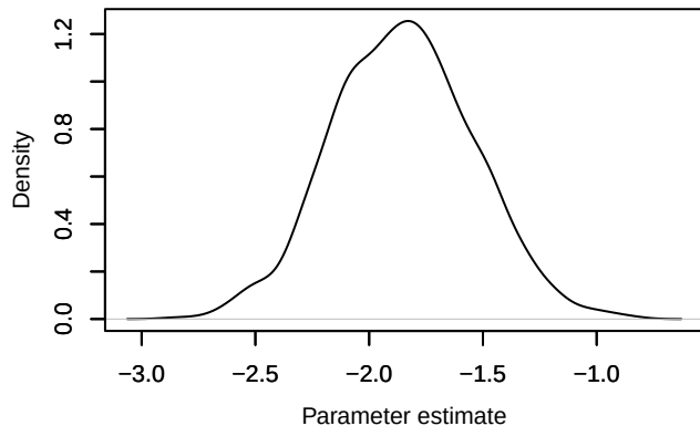
Density – beta1[8]
