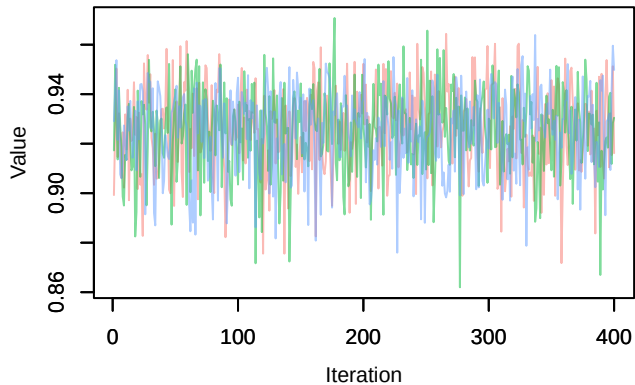
Trace – phi.age[4]
