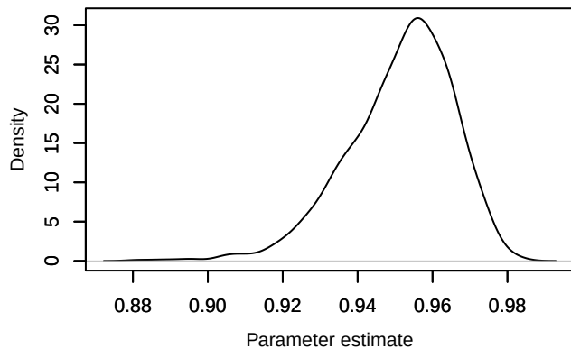
Density – phi.year[3]
