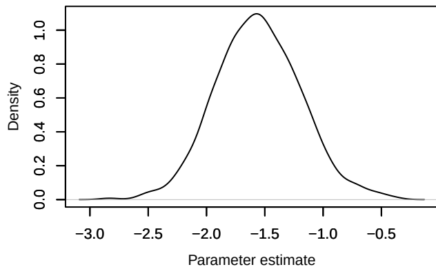
Density – beta1[8]
