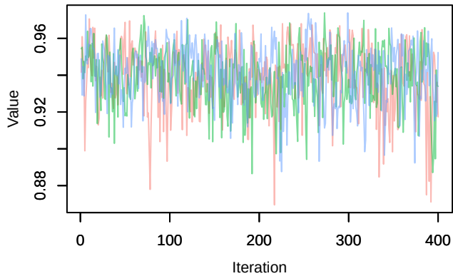
Trace – phi.year[7]
