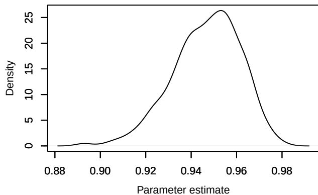
Density – phi.age[6]
