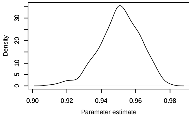
Density – phi.age[3]
