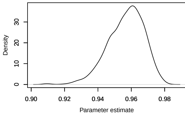
Density – phi.year[1]
