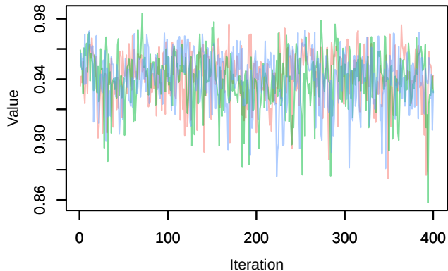
Trace – phi.year[10]
