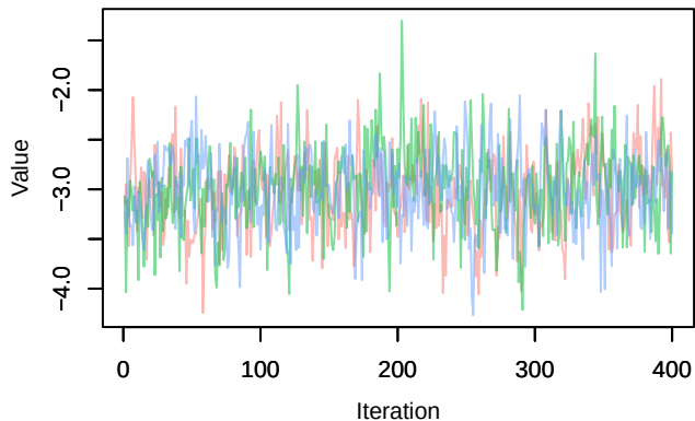
Trace – beta1[11]
