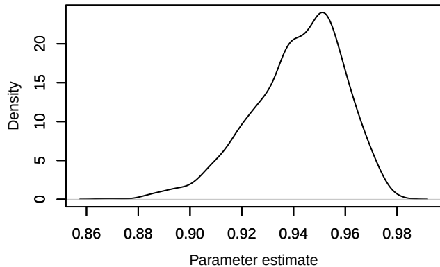
Density – phi.year[10]
