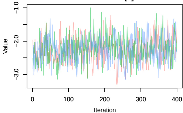
Trace – beta1[10]
