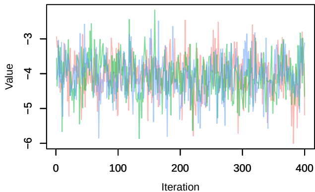
Trace – beta1[11]
