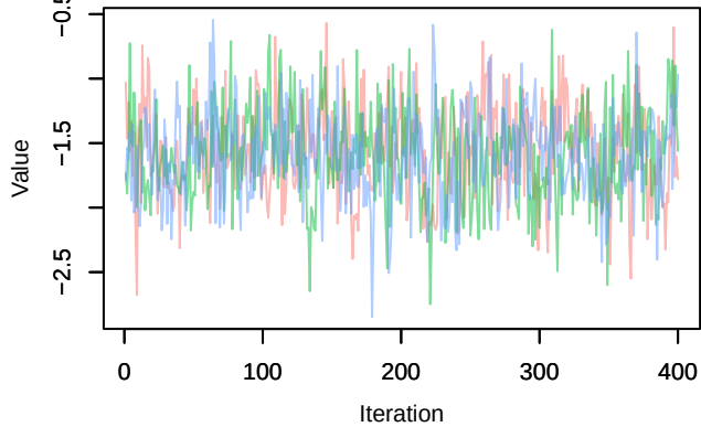
Trace – beta1[8]
