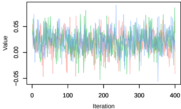
Trace – phi.1diff[5]
