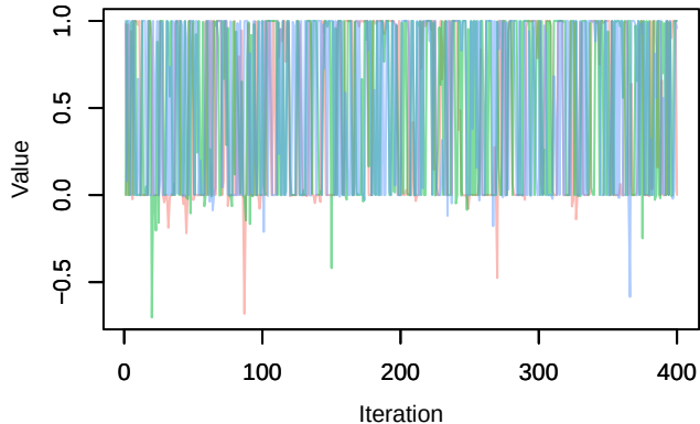
Trace – phi.1diff[14]
