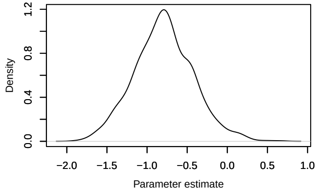
Density – beta1[7]
