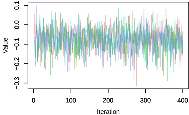
Trace – phi.2diff[10]
