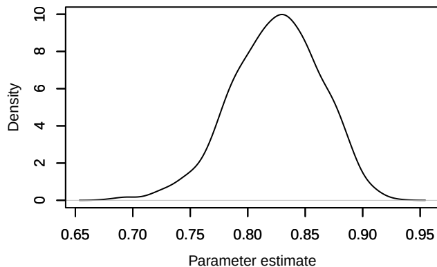
Density – phi.age[8]
