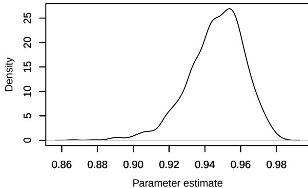
Density – phi.age[5]
