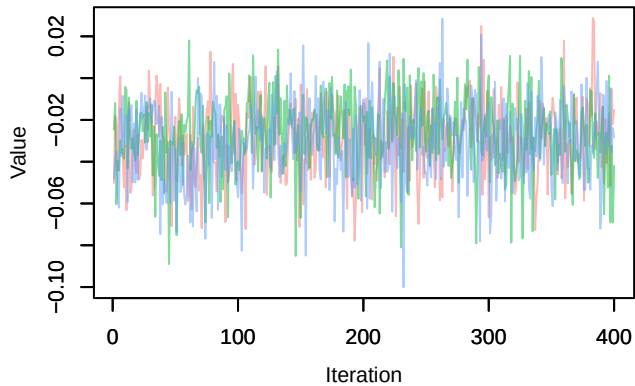
Trace – phi.1diff[5]
