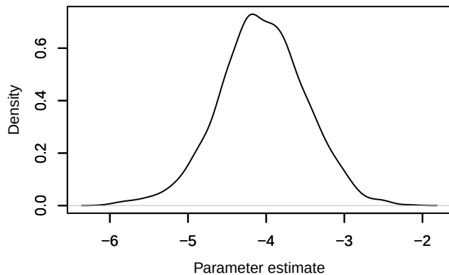
Density – beta1[11]
