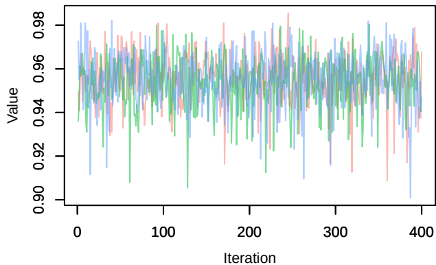
Trace – phi.age[4]
