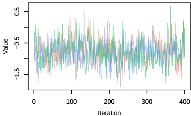
Trace – beta1[7]
