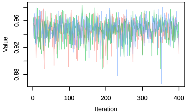
Trace – phi.age[5]
