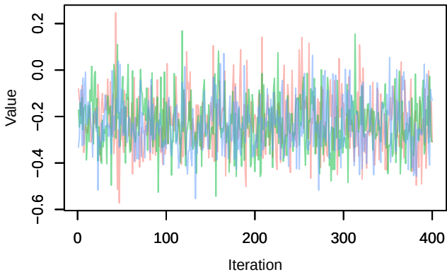
Trace – phi.1diff[11]
