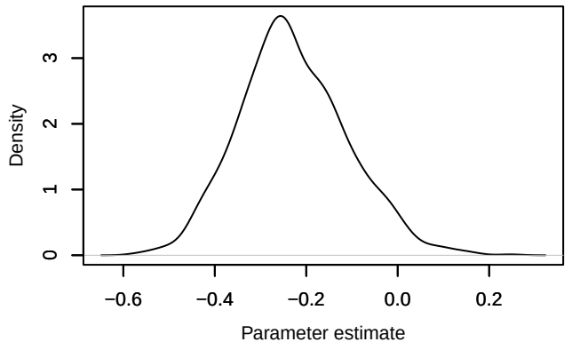
Density – phi.1diff[11]
