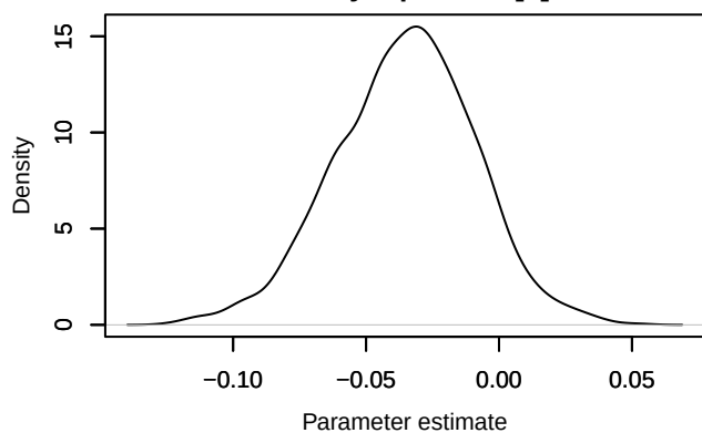
Density – phi.1diff[7]
