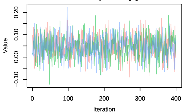
Trace – phi.1diff[8]
