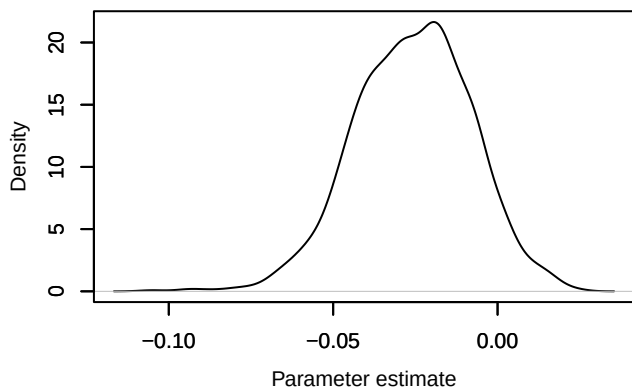
Density – phi.2diff[4]
