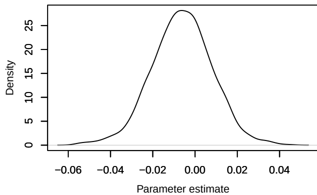
Density – phi.1diff[2]
