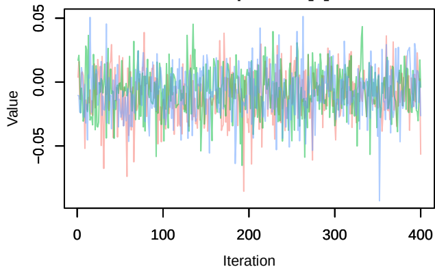
Trace – phi.2diff[6]
