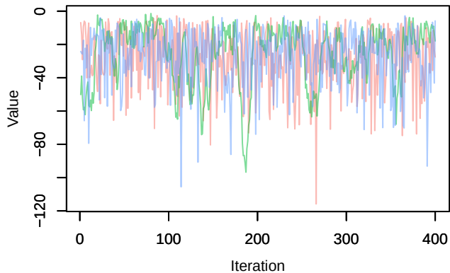
Trace – beta1[13]
