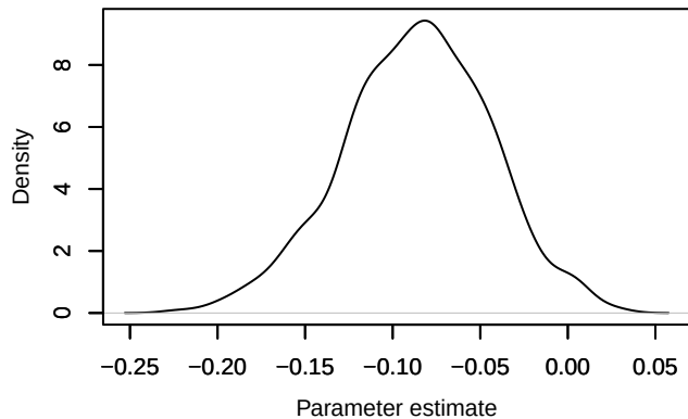
Density – phi.2diff[9]
