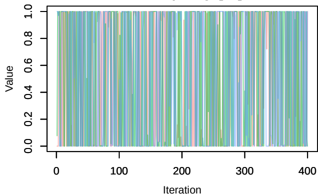
Trace – phi.average
