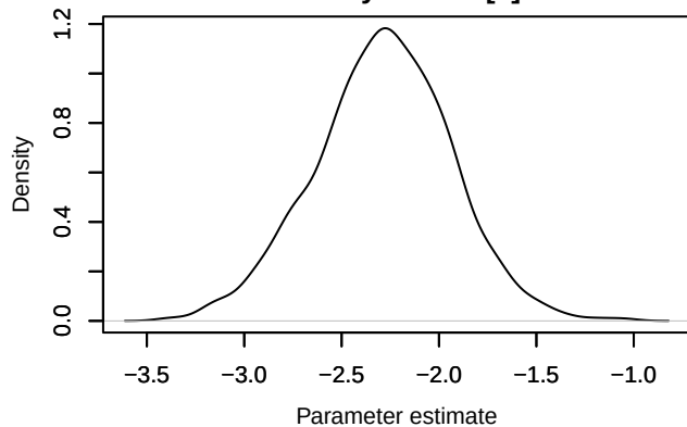
Density – beta1[10]
