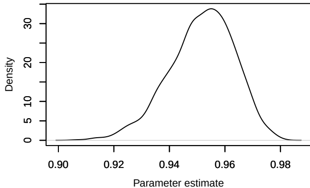
Density – phi.age[2]
