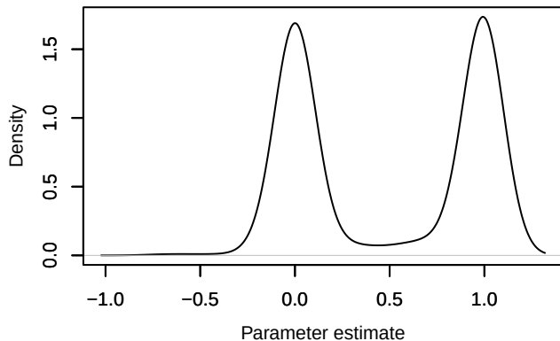
Density – phi.1diff[14]
