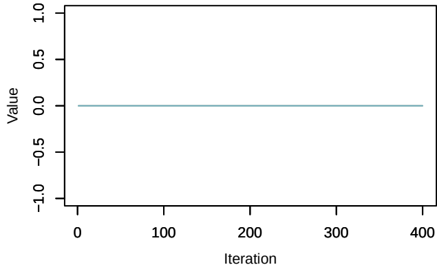
Trace – beta1[2]
