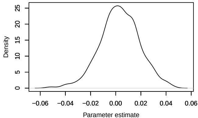
Density – phi.1diff[4]
