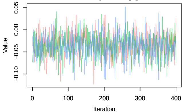
Trace – phi.1diff[7]
