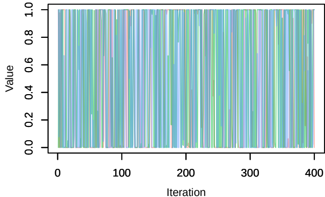
Trace – phi.age[14]
