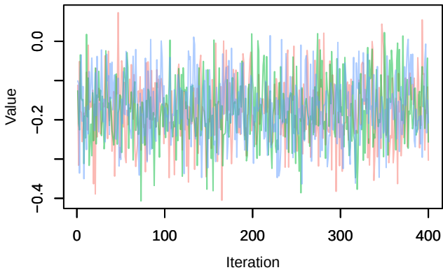
Trace – phi.1diff[11]
