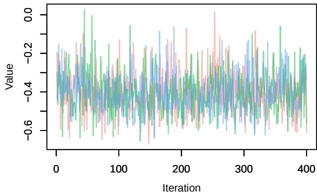
Trace – phi.2diff[12]
