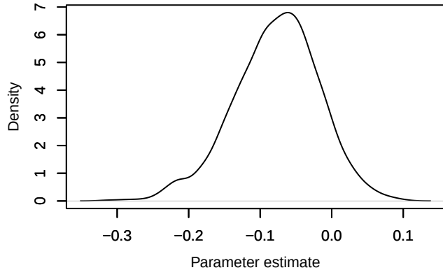
Density – phi.2diff[10]
