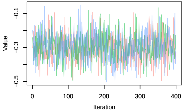
Trace – phi.2diff[10]
