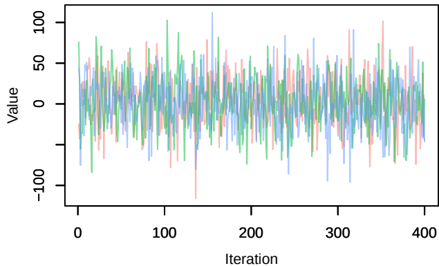
Trace – beta1[14]
