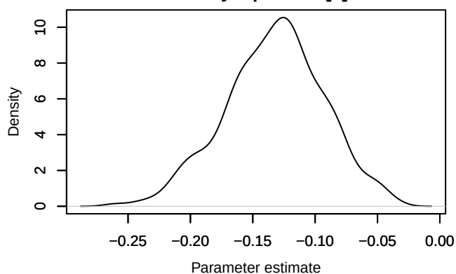
Density – phi.1diff[8]
