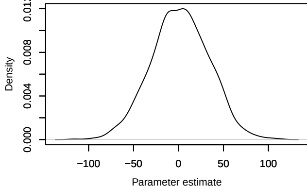
Density – beta1[14]
