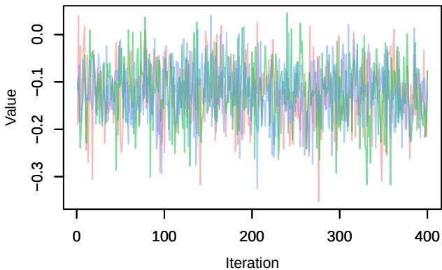
Trace – phi.1diff[10]
