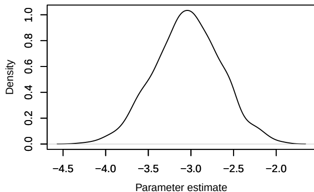
Density – beta1[10]
