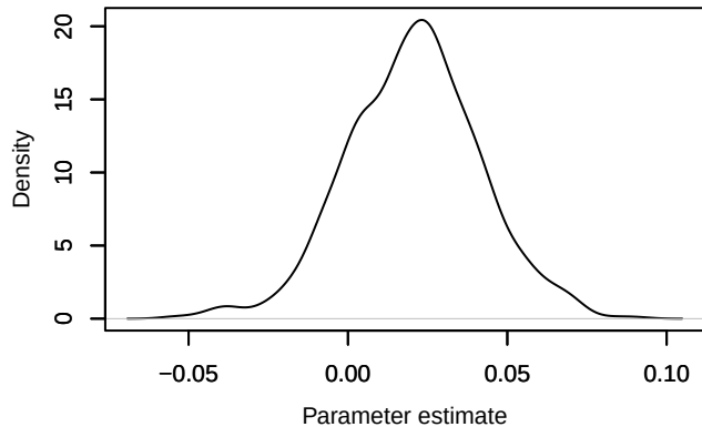
Density – phi.1diff[5]
