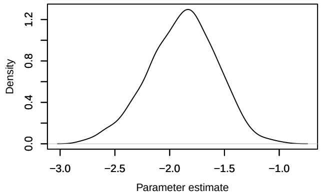
Density – beta1[8]
