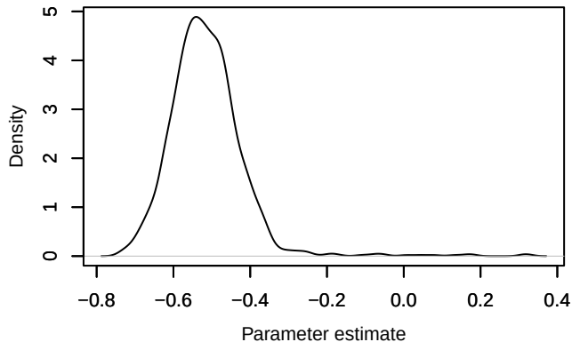
Density – phi.2diff[13]
