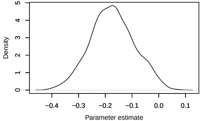
Density – phi.1diff[11]
