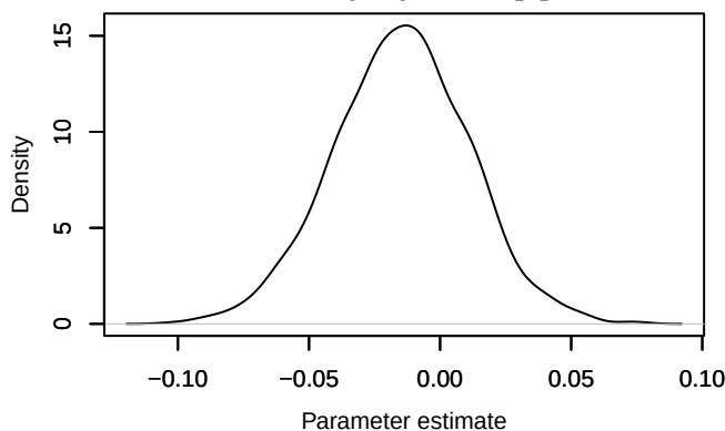
Density – phi.2diff[6]
