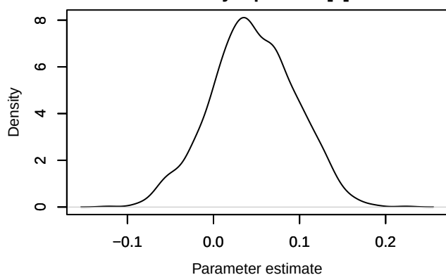
Density – phi.1diff[8]
