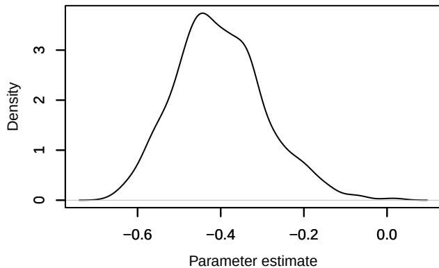
Density – phi.2diff[12]
