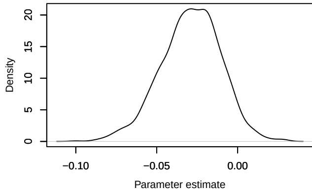
Density – phi.1diff[5]
