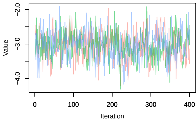
Trace – beta1[10]
