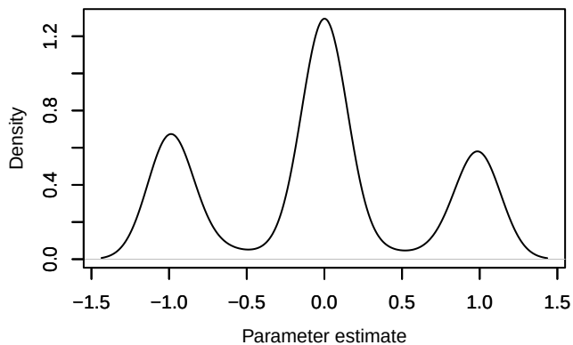
Density – phi.2diff[3]
