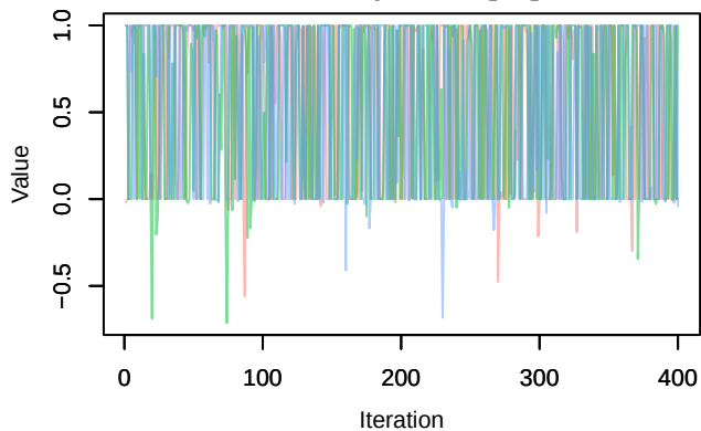
Trace – phi.2diff[15]
