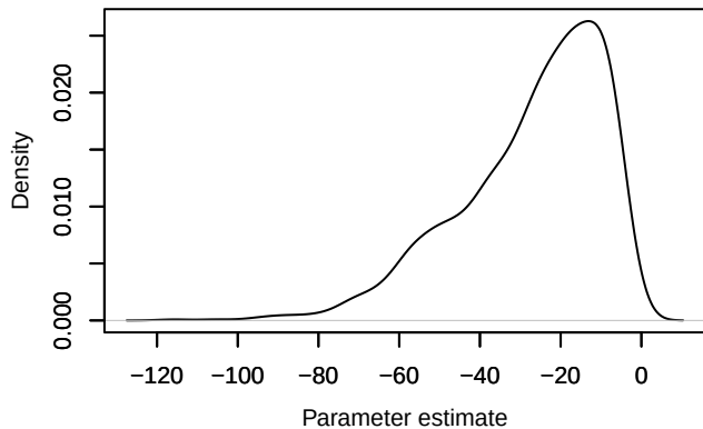
Density – beta1[13]
