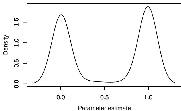
Density – phi.average
