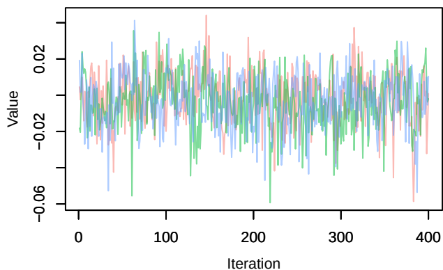
Trace – phi.2diff[3]
