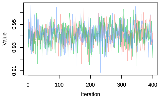
Trace – phi.1diff[2]
