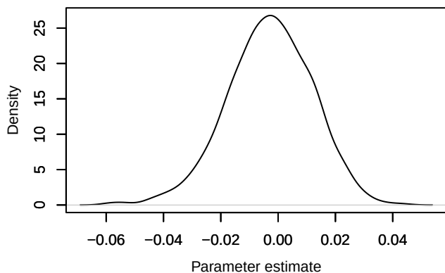
Density – phi.2diff[3]
