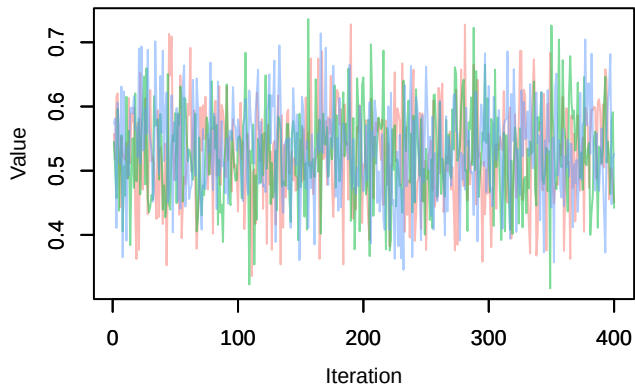
Trace – phi.age[11]
