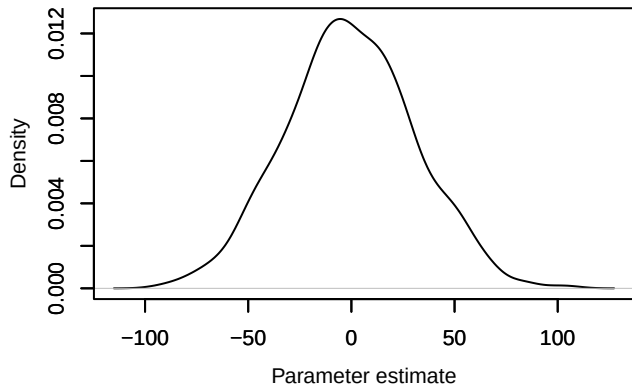
Density – phi.age[1]
