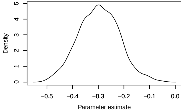
Density – phi.2diff[10]
