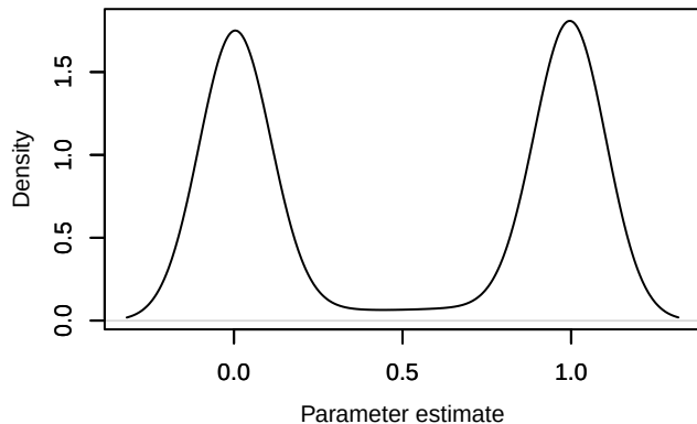
Density – phi.age[14]
