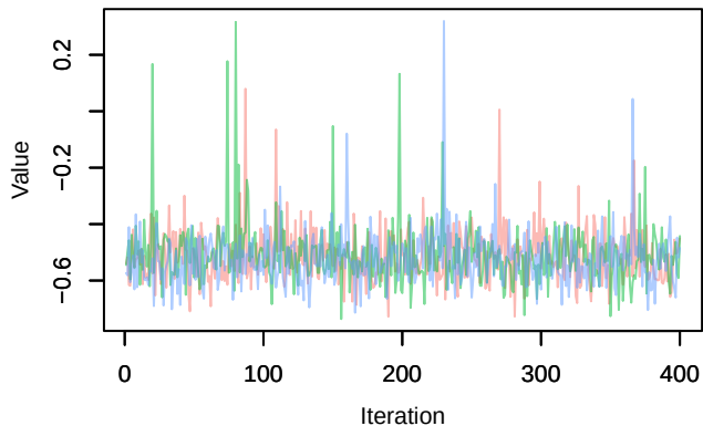
Trace – phi.2diff[13]
