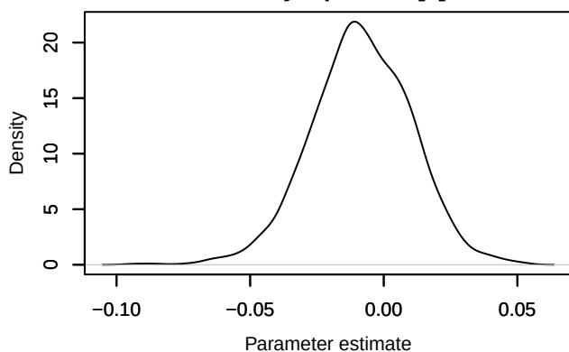
Density – phi.2diff[6]
