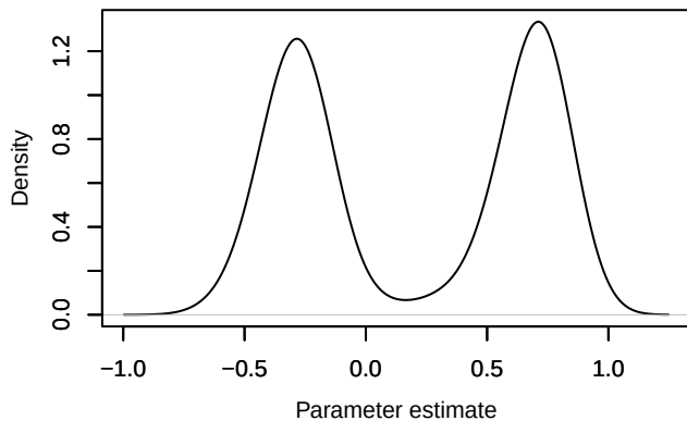
Density – phi.2diff[13]
