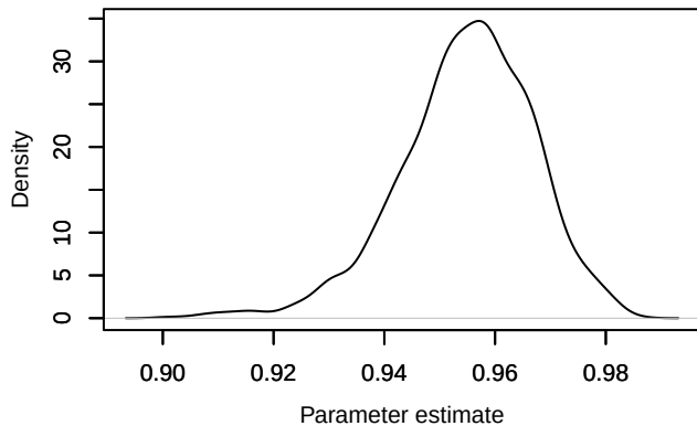
Density – phi.age[4]
