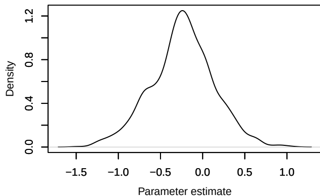
Density – beta1[5]
