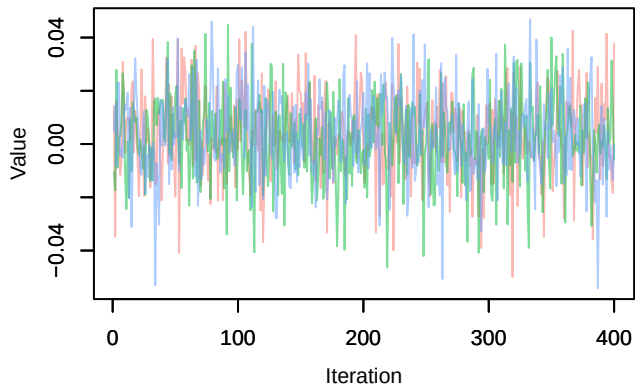
Trace – phi.1diff[4]
