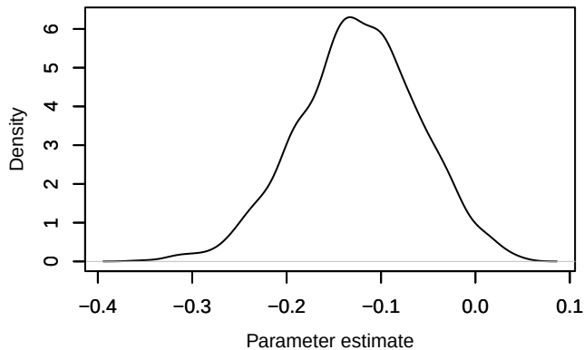
Density – phi.1diff[10]
