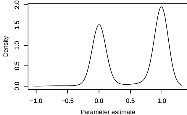
Density – phi.2diff[15]
