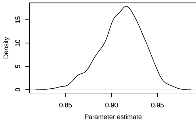
Density – phi.age[7]
