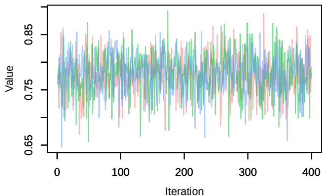
Trace – phi.age[7]
