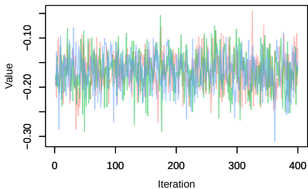
Trace – phi.2diff[7]
