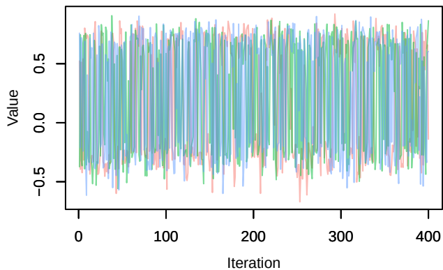
Trace – phi.2diff[13]
