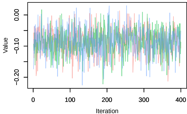
Trace – phi.2diff[9]
