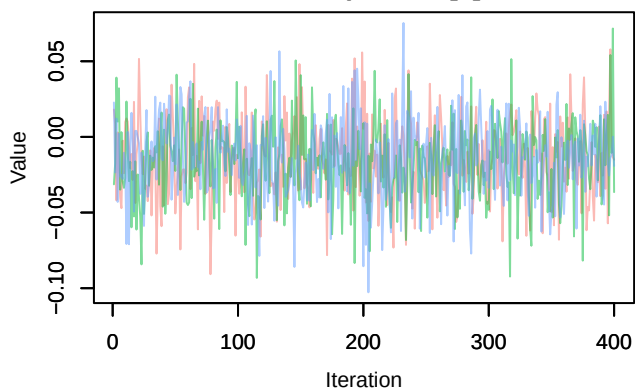
Trace – phi.2diff[6]
