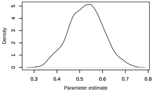
Density – phi.age[11]
