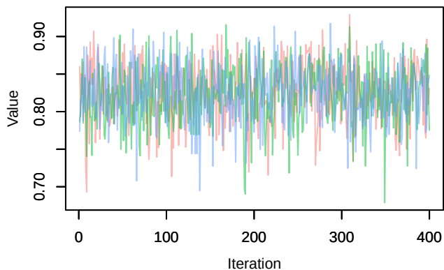
Trace – phi.age[8]
