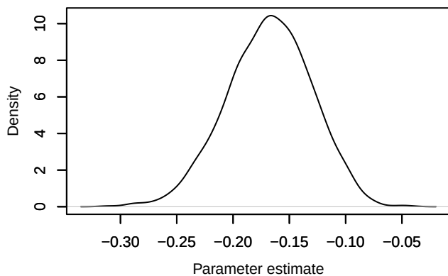
Density – phi.2diff[7]
