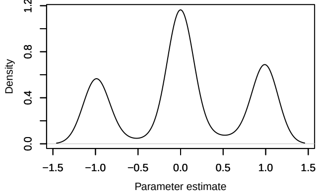
Density – phi.1diff[14]
