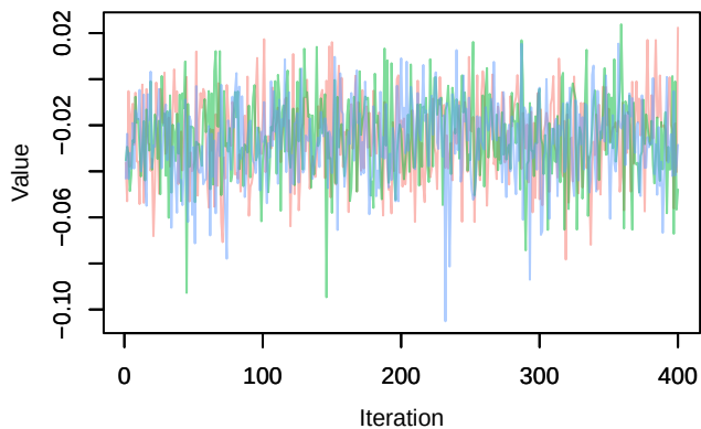
Trace – phi.2diff[4]
