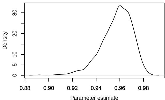
Density – phi.year[1,8]
