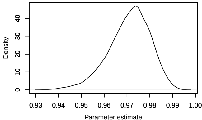
Density – phi.year[2,5]
