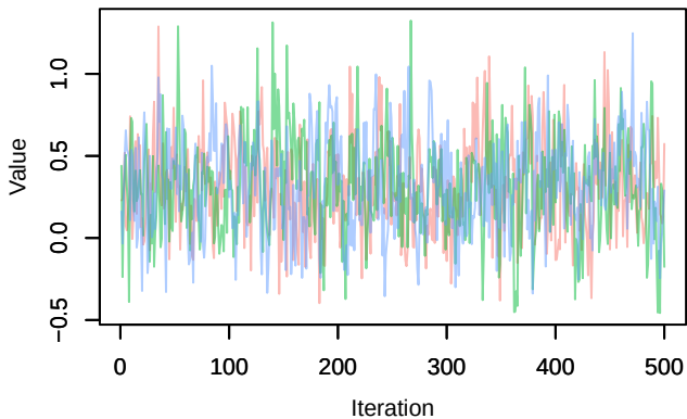
Trace – beta4[1]
