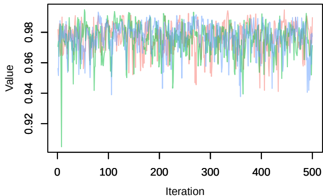
Trace – phi.year[1,4]
