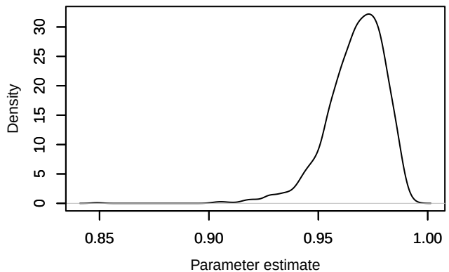
Density – phi.year[2,2]
