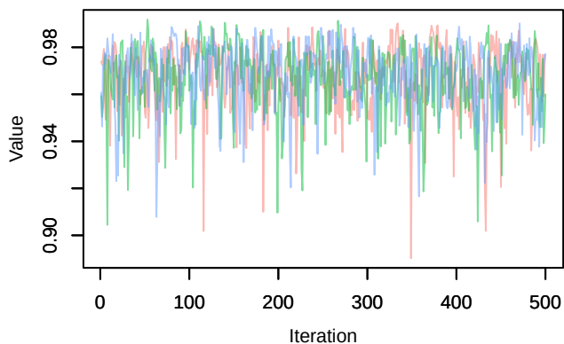
Trace – phi.year[2,8]
