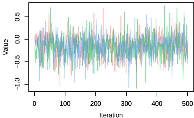
Trace – eps1[11]
