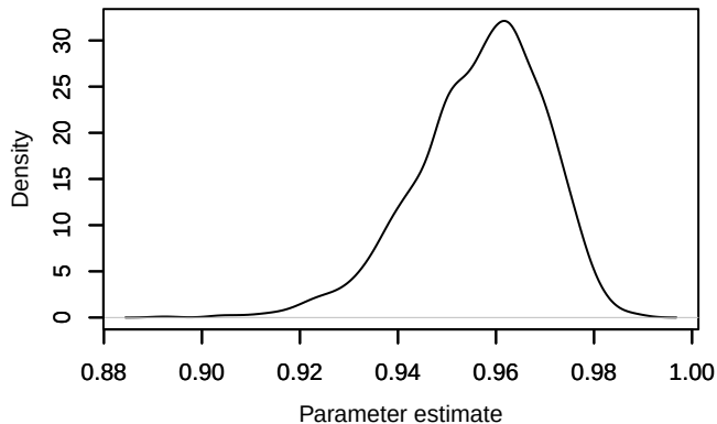
Density – phi.year[2,2]
