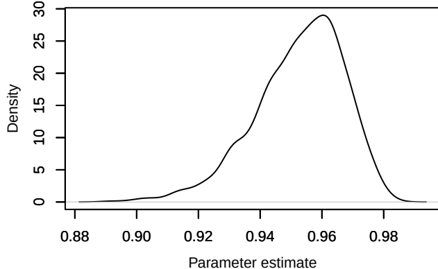
Density – phi.year[1,7]
