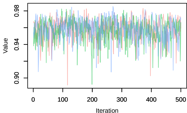
Trace – phi.year[1,8]
