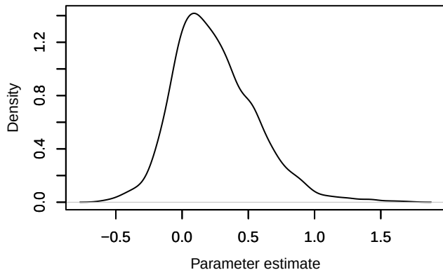
Density – eps1[12]
