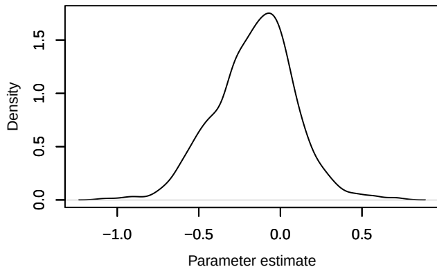
Density – eps1[11]
