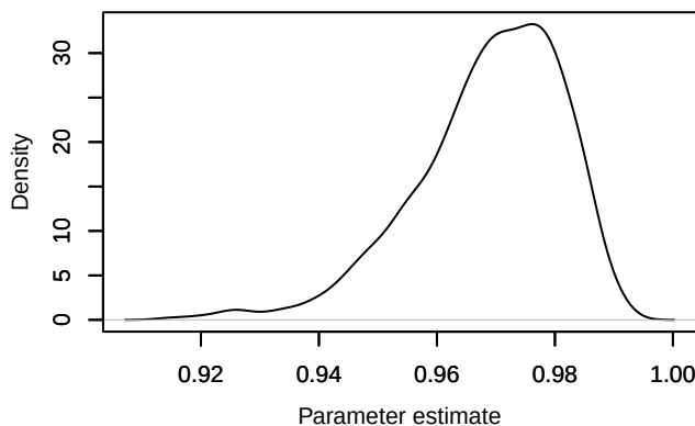
Density – phi.year[2,6]
