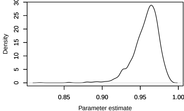
Density – phi.year[1,13]
