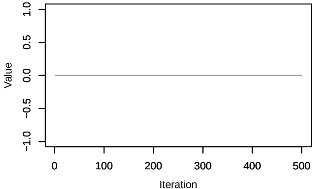
Trace – beta4[2]
