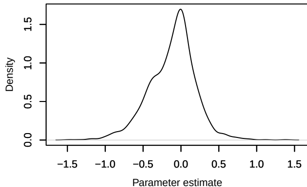
Density – eps1[14]
