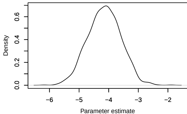
Density – beta1[11]
