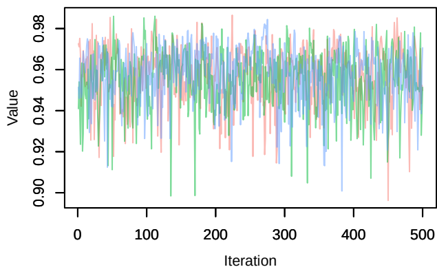
Trace – phi.year[1,10]
