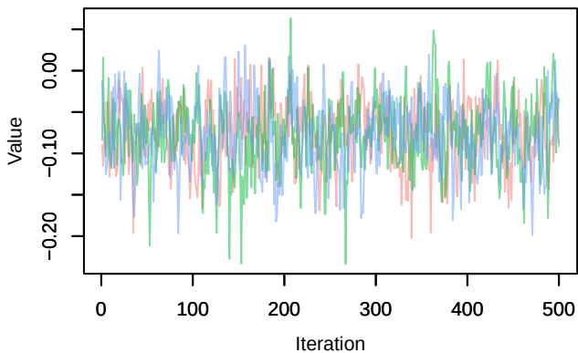
Trace – beta4[2]
