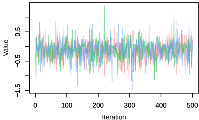
Trace – eps1[14]
