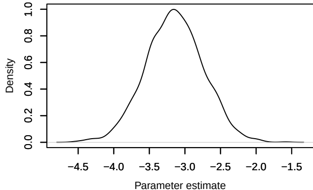
Density – beta1[11]
