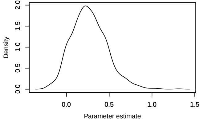
Density – eps1[6]
