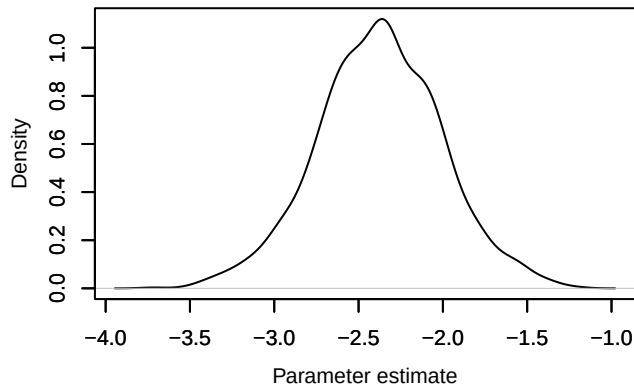
Density – beta1[10]
