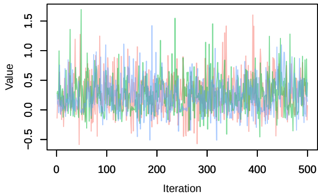
Trace – eps1[12]
