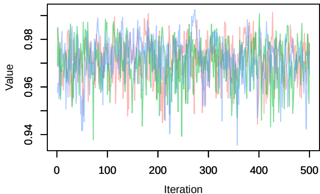
Trace – phi.year[2,5]
