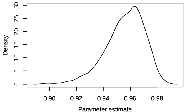
Density – phi.year[1,10]
