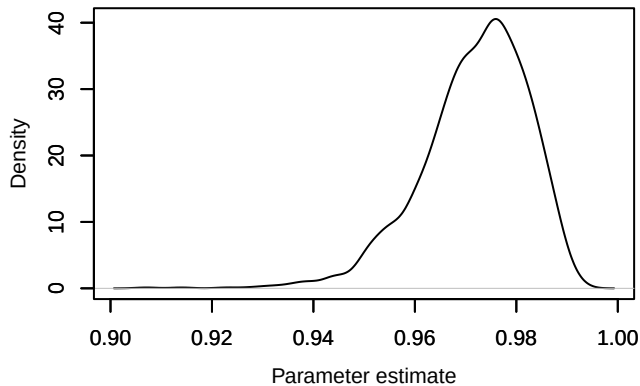
Density – phi.year[1,2]
