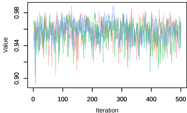
Trace – phi.year[2,2]
