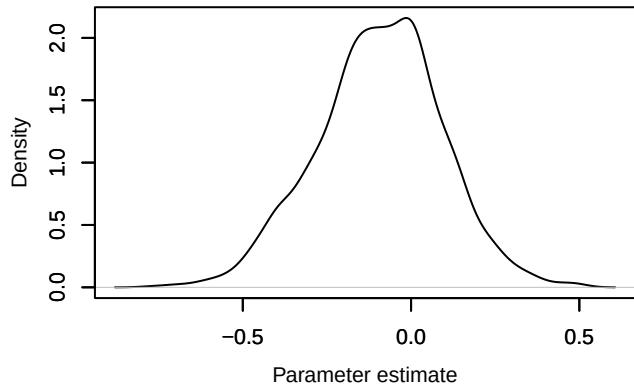
Density – eps1[6]
