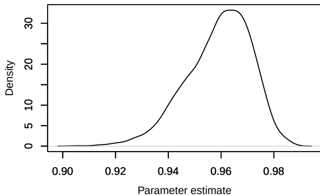
Density – phi.year[1,6]
