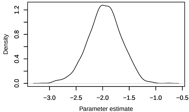
Density – beta1[8]
