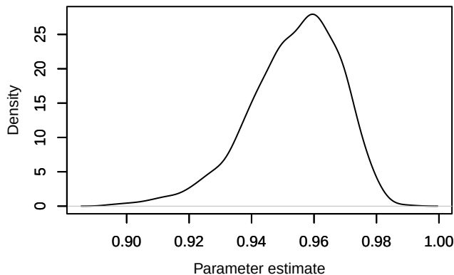
Density – phi.year[1,9]
