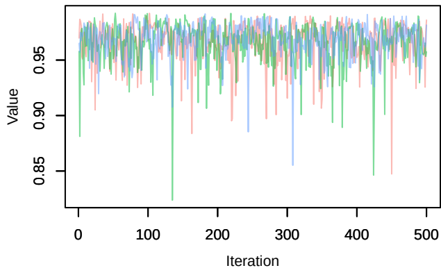
Trace – phi.year[1,14]
