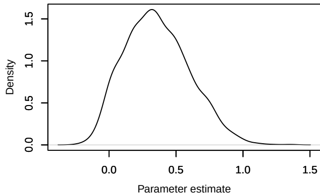
Density – eps1[5]
