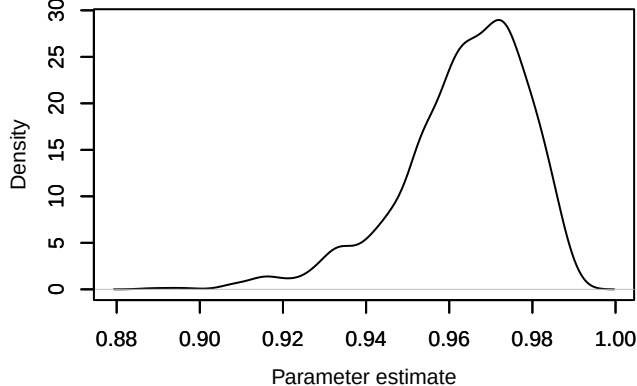
Density – phi.year[2,7]
