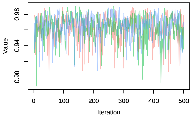
Trace – phi.year[2,7]
