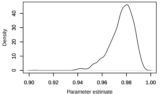
Density – phi.year[1,4]
