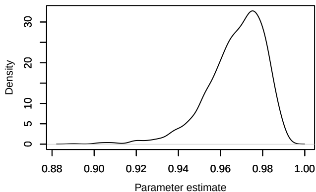
Density – phi.year[2,8]
