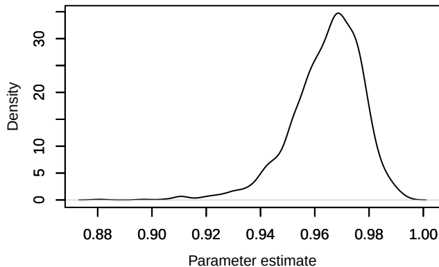
Density – phi.year[2,12]
