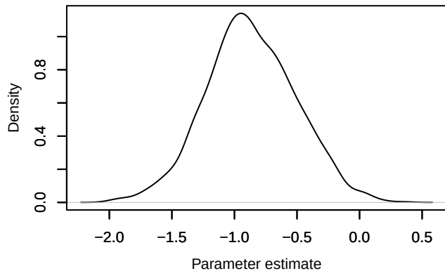
Density – beta1[7]
