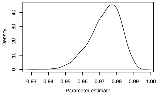
Density – phi.year[1,4]
