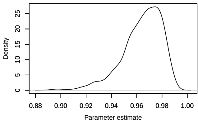
Density – phi.year[2,9]
