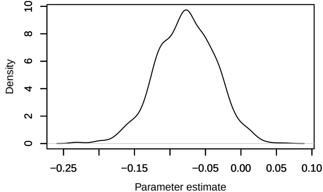
Density – beta4[2]
