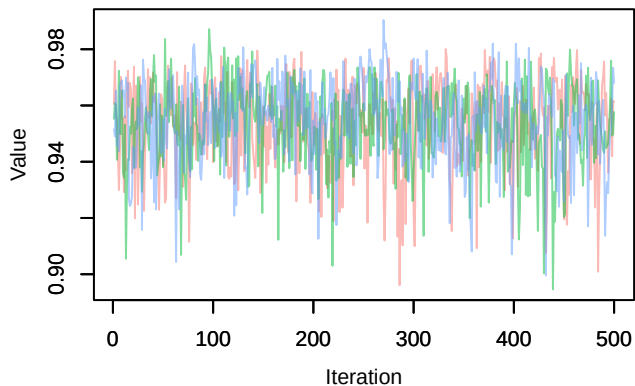
Trace – phi.year[1,9]
