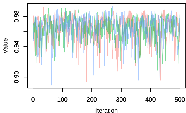
Trace – phi.year[2,9]
