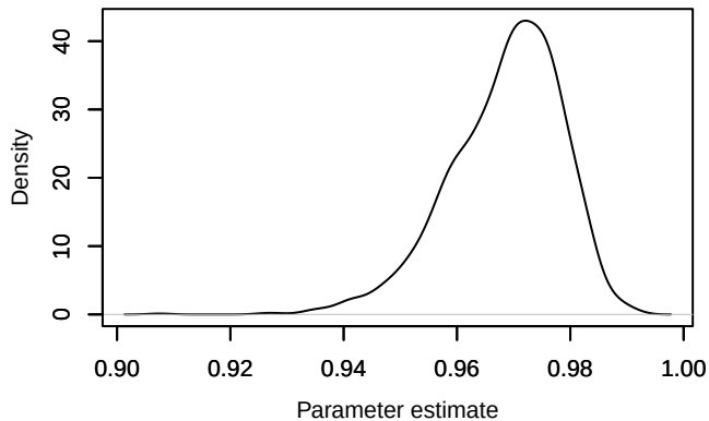
Density – phi.year[2,3]
