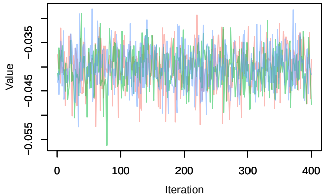
Trace – phi_diff[7]
