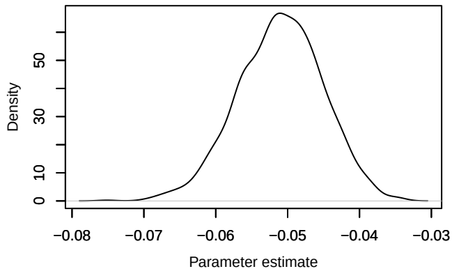
Density – phi_diff[9]
