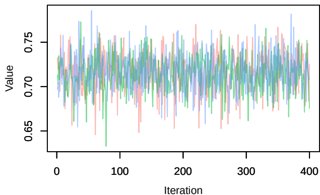
Trace – phi.age[9]
