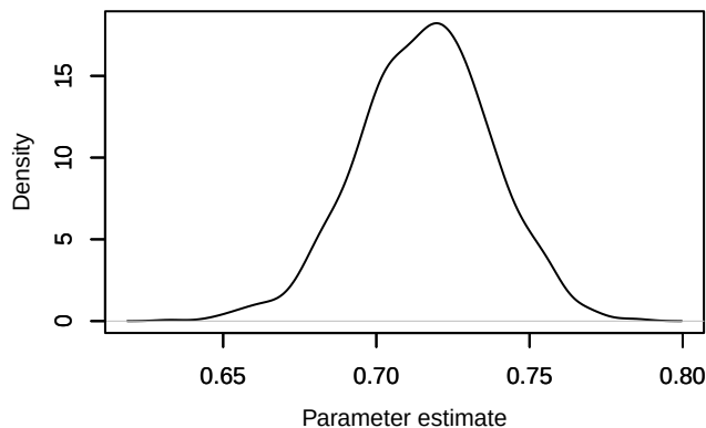
Density – phi.age[9]
