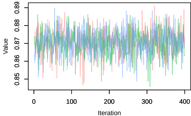
Trace – phi.age[6]
