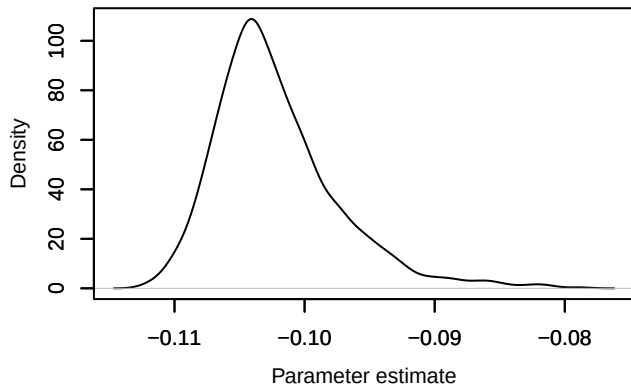
Density – phi_diff[15]
