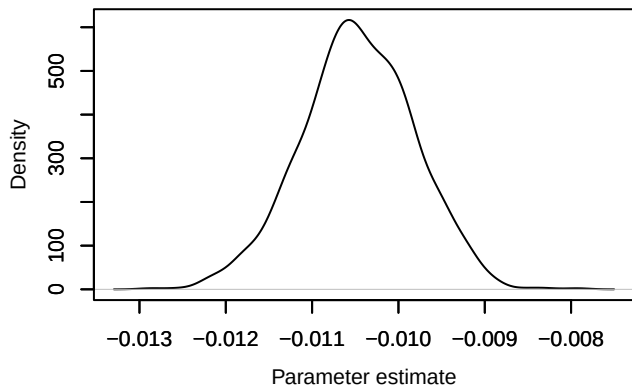
Density – phi_diff[3]
