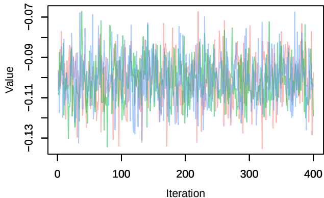
Trace – phi_diff[12]
