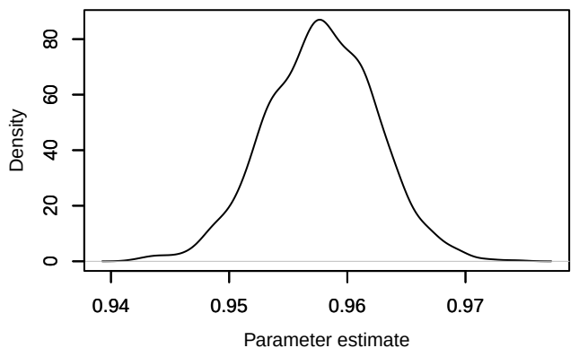
Density – phi.age[2]
