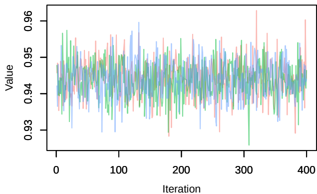
Trace – phi.age[3]
