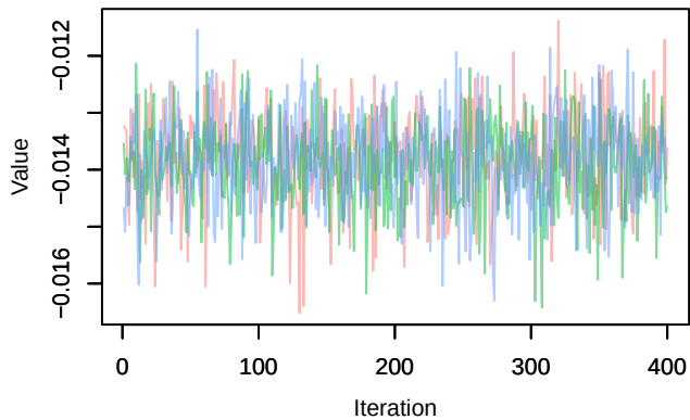
Trace – phi_diff[4]
