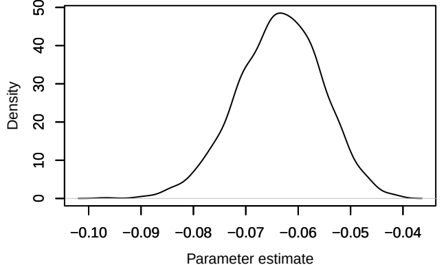
Density – phi_diff[10]
