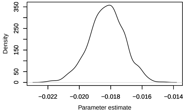
Density – phi_diff[4]
