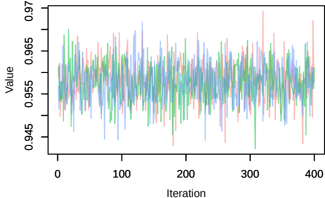
Trace – phi.age[2]
