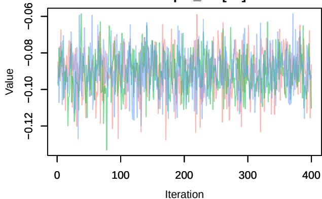
Trace – phi_diff[12]
