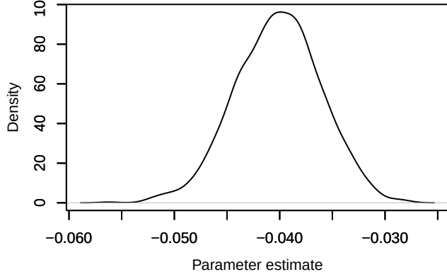
Density – phi_diff[7]
