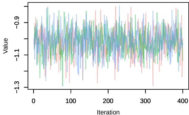
Trace – age_decline
