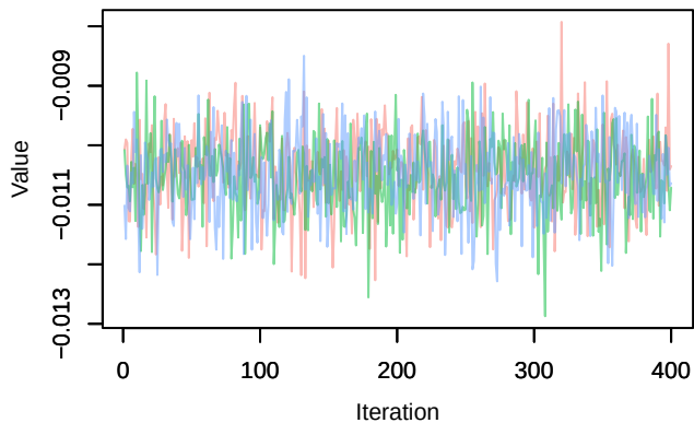
Trace – phi_diff[3]
