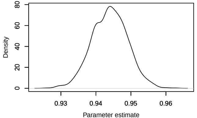
Density – phi.age[3]
