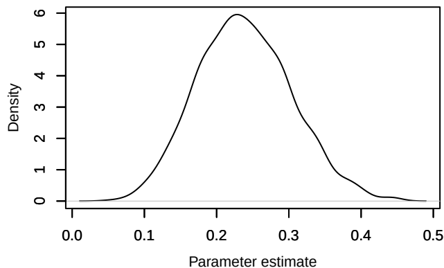
Density – phi.age[15]
