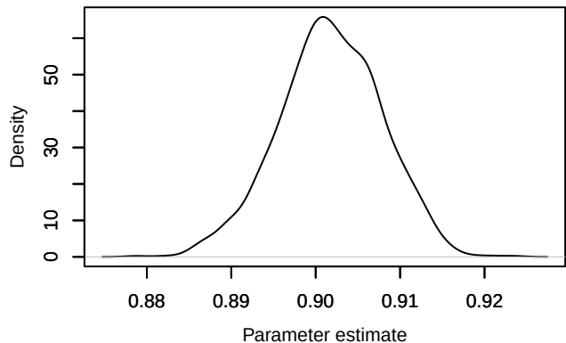
Density – phi.age[6]
