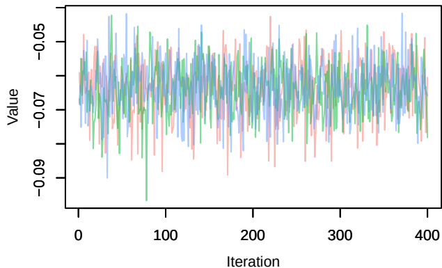
Trace – phi_diff[10]
