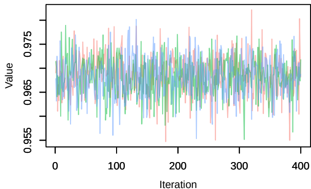
Trace – phi.age[1]
