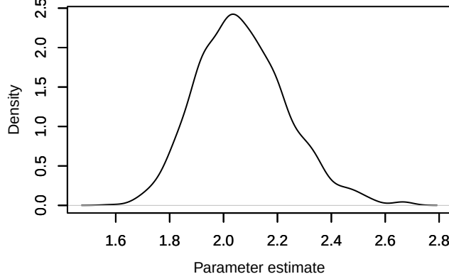
Density – age_decline
