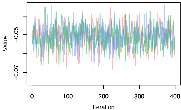
Trace – phi_diff[9]
