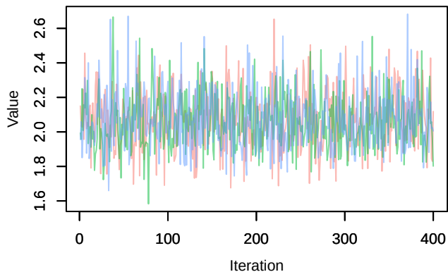
Trace – age_decline
