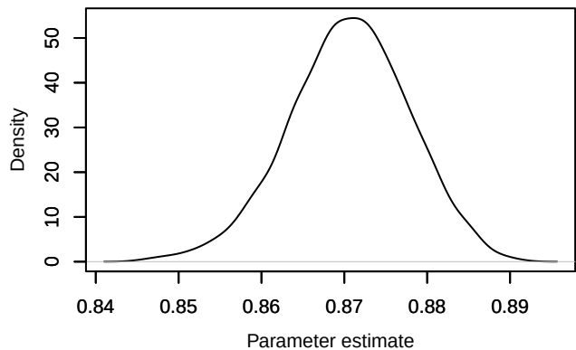
Density – phi.age[6]
