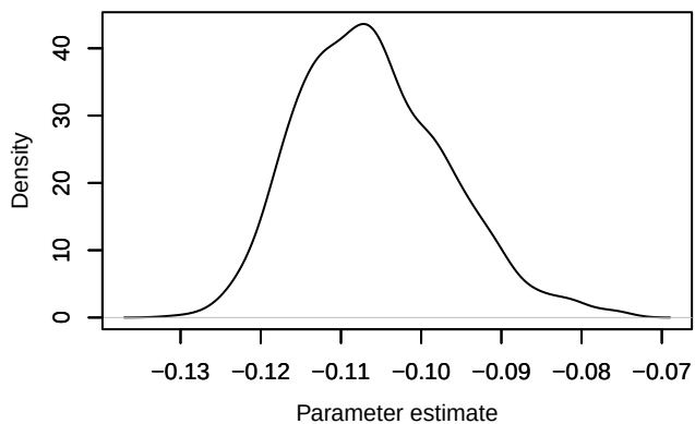
Density – phi_diff[13]
