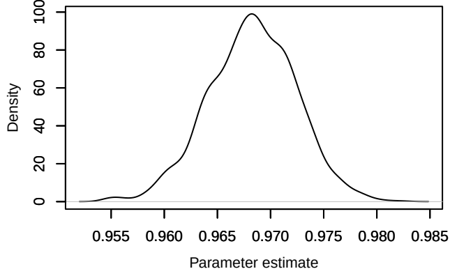
Density – phi.age[1]
