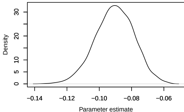
Density – phi_diff[12]
