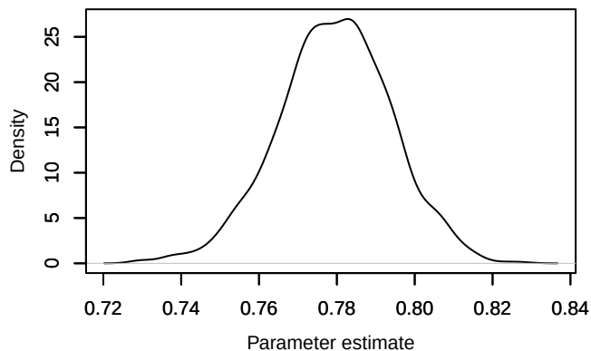
Density – phi.age[8]
