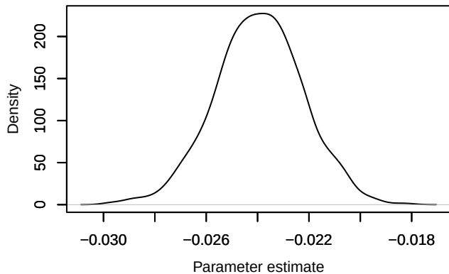
Density – phi_diff[6]
