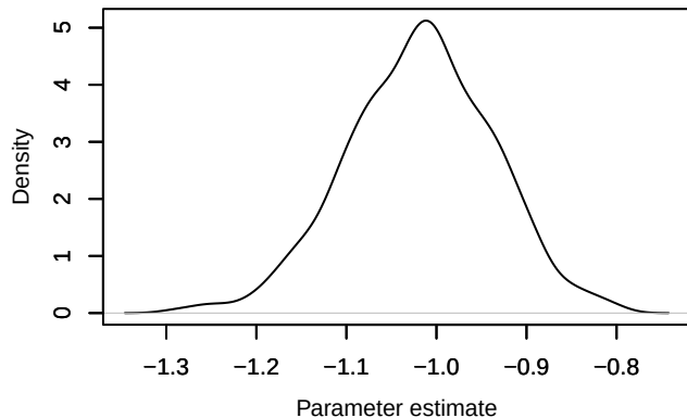
Density – age_decline
