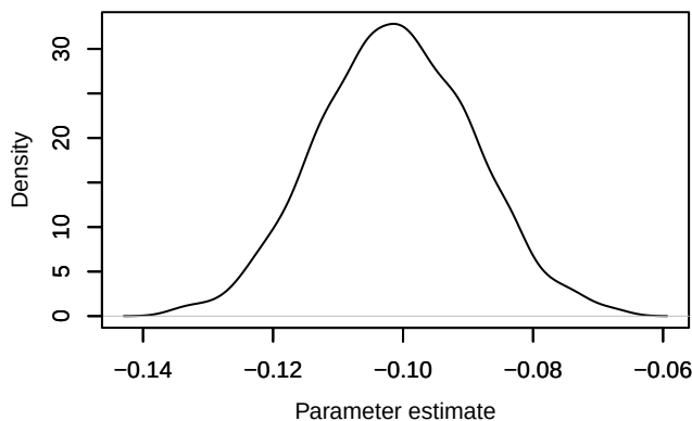
Density – phi_diff[12]
