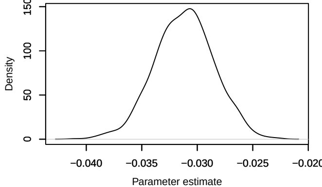
Density – phi_diff[7]
