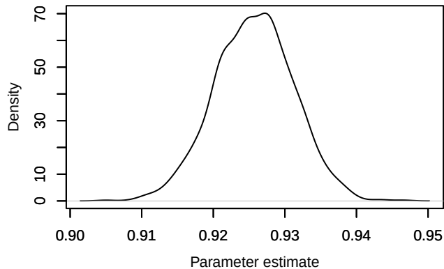
Density – phi.age[5]
