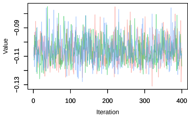
Trace – phi_diff[13]
