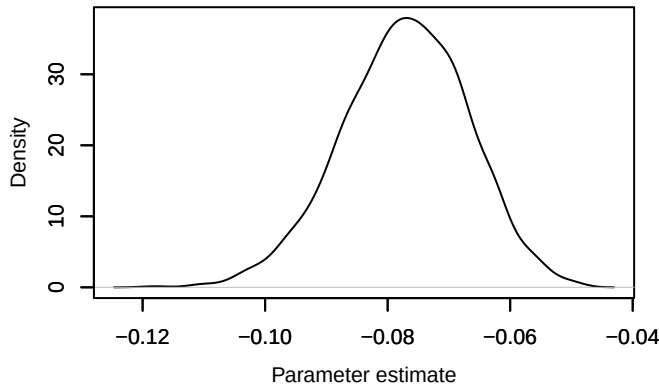
Density – phi_diff[10]
