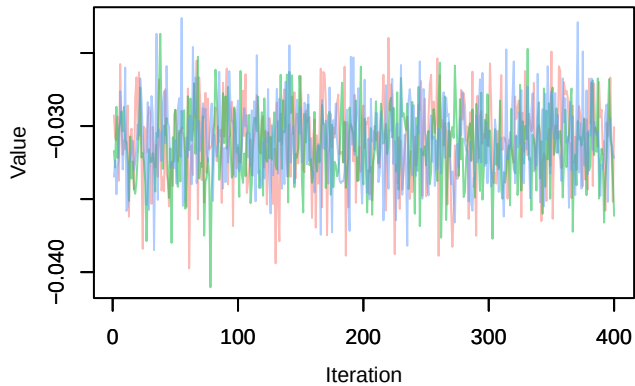
Trace – phi_diff[7]
