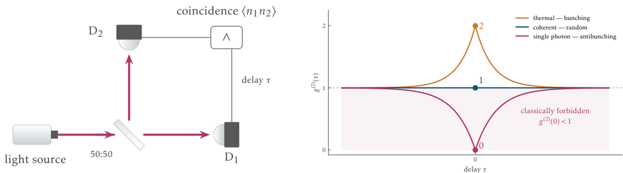
Figure 3: Left: HBT setup — beam splitter, two detectors, coincidence counter. Right: g^{(2)}(\tau) for thermal, coherent, and single-photon light; the shaded region g^{(2)}(0) < 1 is classically forbidden.
