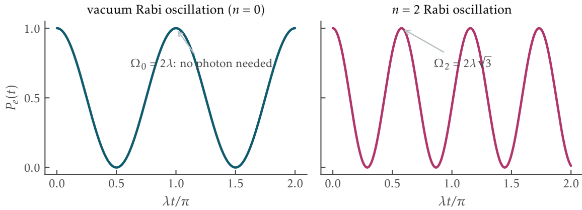
Figure 4: Jaynes–Cummings Rabi oscillations, P_e(t) = \cos^2(\lambda\sqrt{n+1}t) , for n = 0 (vacuum) and n = 2 ; the oscillation persists at n = 0 .
