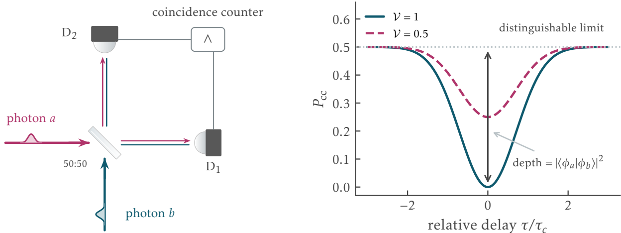
Figure 2: The Hong–Ou–Mandel effect. Left: two single photons meet at a 50:50 beam splitter; a coincidence counter monitors the two outputs. Right: coincidence probability vs. relative delay, Eq. (1.10): identical photons give a dip to zero; partial distinguishability ( \nu = |\langle \phi_a | \phi_b \rangle|^2 = 0.5 shown) makes the dip shallower.
