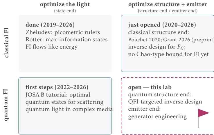
Figure 6: The state of the field, as a map. Both classical lines and the quantum first steps optimize the light ; the classical structure end has just opened; the quantum structure end and the emitter end (flag) are this lab’s claim.
