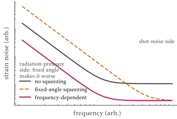
Figure 3: Why the squeezing angle must rotate with frequency (schematic noise budget, after Ref. [5]). Fixed-angle squeezing lowers shot noise but raises radiation-pressure noise; frequency-dependent squeezing lowers both.
