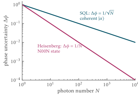
Figure 4: The two scalings of phase estimation, Eqs. (2.4) and (2.6). The gap between them is what “quantum-enhanced sensing” means.
