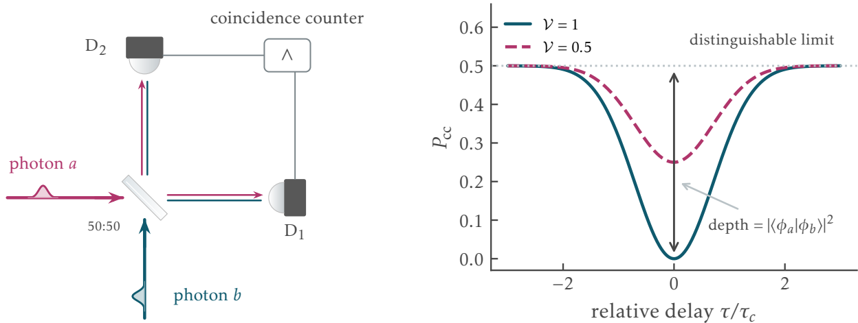
Figure 2: The Hong–Ou–Mandel effect. Left: two single photons meet at a 50:50 beam splitter; a coincidence counter monitors the two outputs. Right: coincidence probability vs. relative delay, Eq. (1.10): identical photons give a dip to zero; partial distinguishability ( \mathcal{V} = |\langle \phi_a | \phi_b \rangle|^2 = 0.5 shown) makes the dip shallower.
