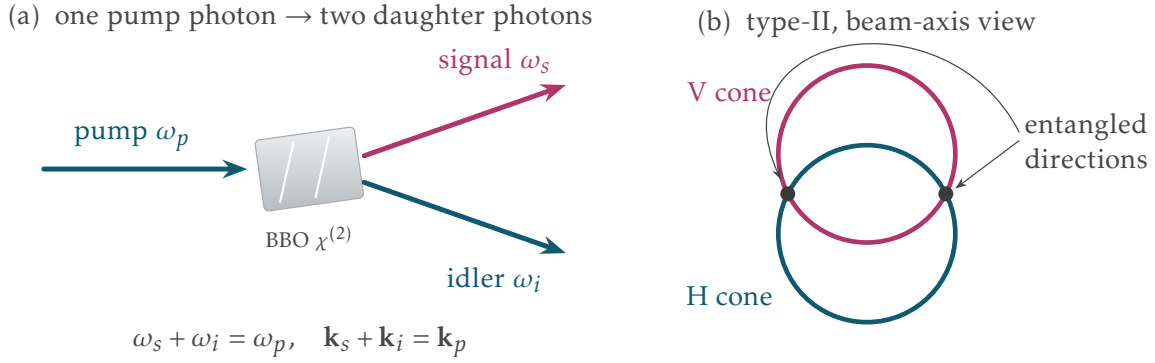
Figure 1: Spontaneous parametric down-conversion. (a) One pump photon splits into a signal-idler pair in a \chi^{(2)} crystal, constrained by energy and momentum conservation, Eq. (1.2). (b) Type-II phase matching: the orthogonally polarized cones intersect along two directions, where the pair is polarization entangled, Eq. (1.6).
