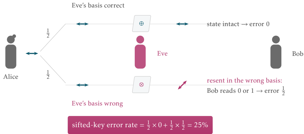
Figure 4: Intercept-resend attack on BB84. Eve's basis guess is right half the time (no disturbance) and wrong half the time (Bob's sifted bit is random), producing a 25% error rate in the sifted key, Eq. (3.2).
