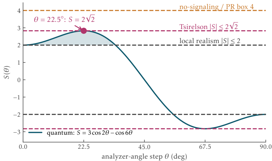
Figure 3: CHSH parameter S for the quantum state (|HH\rangle + |VV\rangle)/\sqrt{2} with settings (a, a', b, b') = (0, 2\theta, \theta, 3\theta) , for which S(\theta) = 3 \cos 2\theta - \cos 6\theta . Local realism caps |S| at 2 (grey); quantum mechanics reaches, but never exceeds, 2\sqrt{2} at \theta = 22.5^\circ (Tsirelson bound, magenta).
