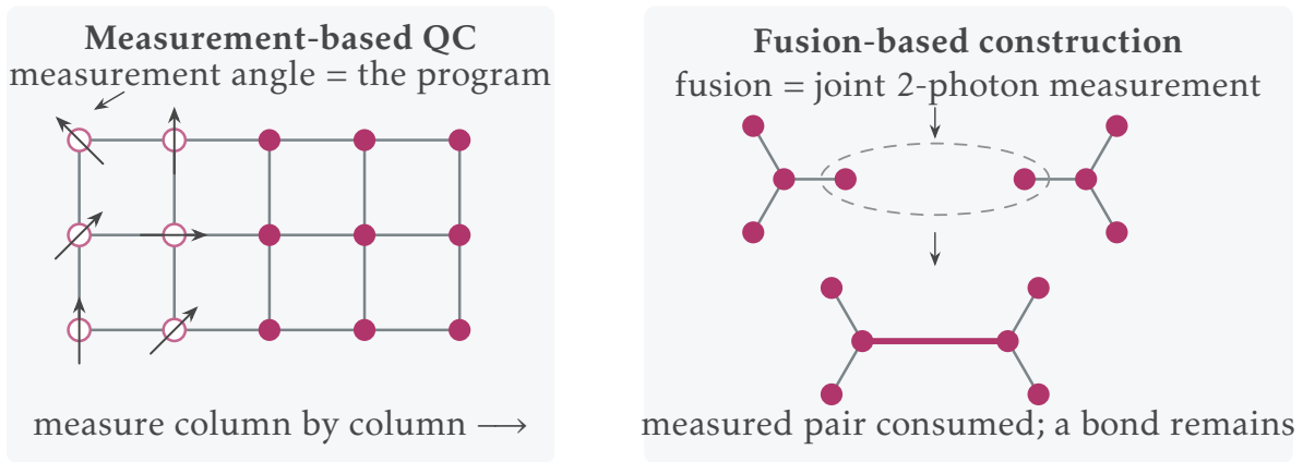
Figure 3: Left: MBQC — entangle first (bonds), then compute by measuring single qubits at program-defined angles. Right: fusion-based construction — small seed states are stitched into the lattice by two-photon fusion measurements; the measured pair is consumed and leaves a bond (after Bartolucci et al. , Nat. Commun. 14 , 912 (2023)).
