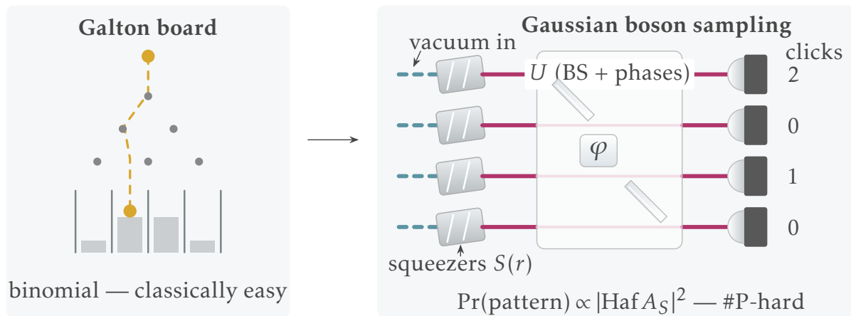
Figure 4: Balls \rightarrow photons, pegs \rightarrow beam splitters. Left: classical Galton board, binomial output. Right: GBS — squeezed vacuum enters a programmable interferometer U ; photon-number-resolved click patterns are distributed according to a #P-hard hafnian, Eq. (2.1). Layout after Madsen et al. , Nature 606 , 75 (2022), Fig. 1.
