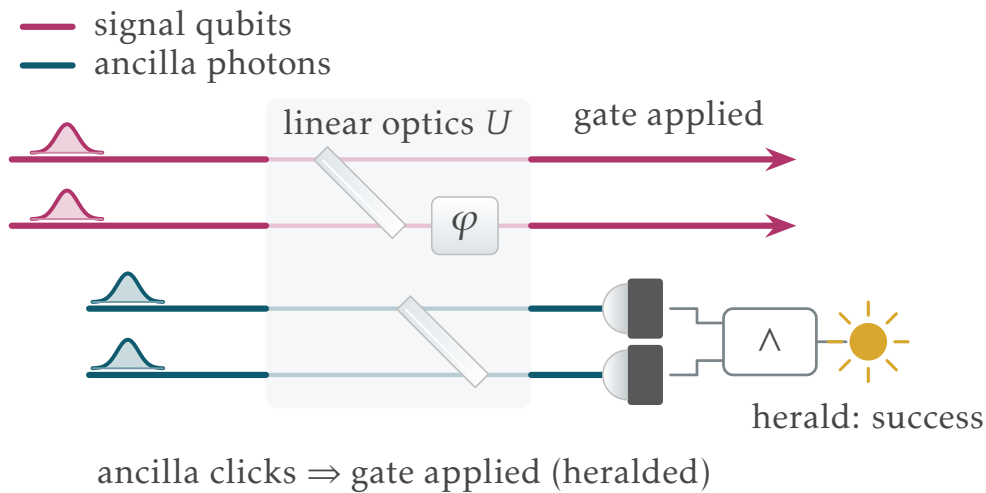
Figure 2: Measurement-induced nonlinearity. Signal qubits and ancilla photons mix in a linear network; a coincidence of ancilla detections heralds success, and only then is the (nonlinear) gate accepted. Layout after Kok et al. , Rev. Mod. Phys. 79 , 135 (2007).
