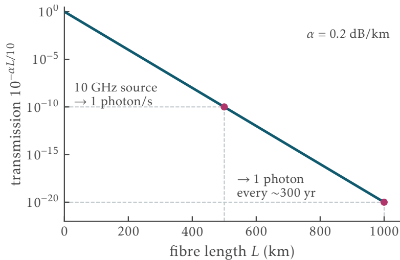
Figure 5: Direct transmission through telecom fiber, Eq. (3.1). The exponential wall is why long-distance quantum communication needs repeaters or satellites, not better lasers.
