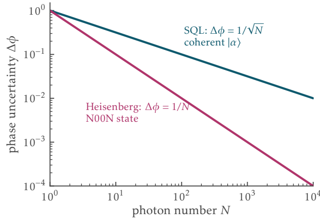
Figure 4: The two scalings of phase estimation, Eqs. (2.4) and (2.6). The gap between them is what “quantum-enhanced sensing” means.
