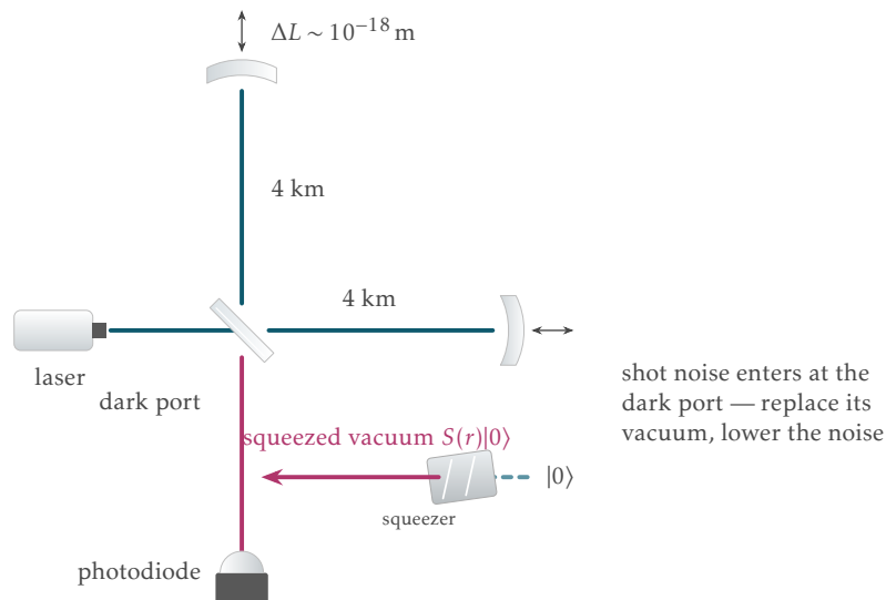
Figure 2: The dark port is where the vacuum — and therefore the shot noise — enters a Michelson interferometer. Replacing that vacuum with squeezed vacuum is how LIGO measures below the SQL.
