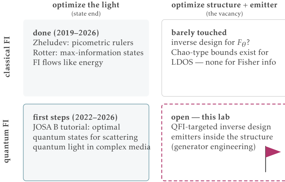
Figure 6: The state of the field, as a map. Both classical lines and the quantum first steps optimize the light ; the structure-and-emitter column is open. The flag is this lab’s claim.
