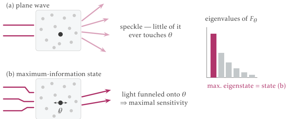
Figure 7: The toy model, Eq. (3.2) (after Ref. [11]). A plane wave wastes most of its light on modes that never touch the parameter \theta ; the top eigenvector of F_\theta funnels everything onto it.
