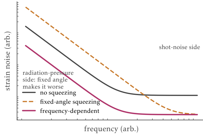
Figure 3: Why the squeezing angle must rotate with frequency (schematic noise budget, after Ref. [4]). Fixed-angle squeezing lowers shot noise but raises radiation-pressure noise; frequency-dependent squeezing lowers both.
