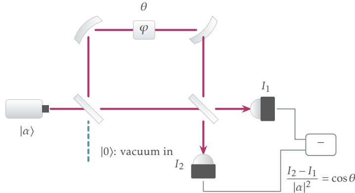
Figure 1: Phase readout with a Mach-Zehnder interferometer. The unused input port is not idle: its vacuum fluctuations are the noise floor of the measurement.
