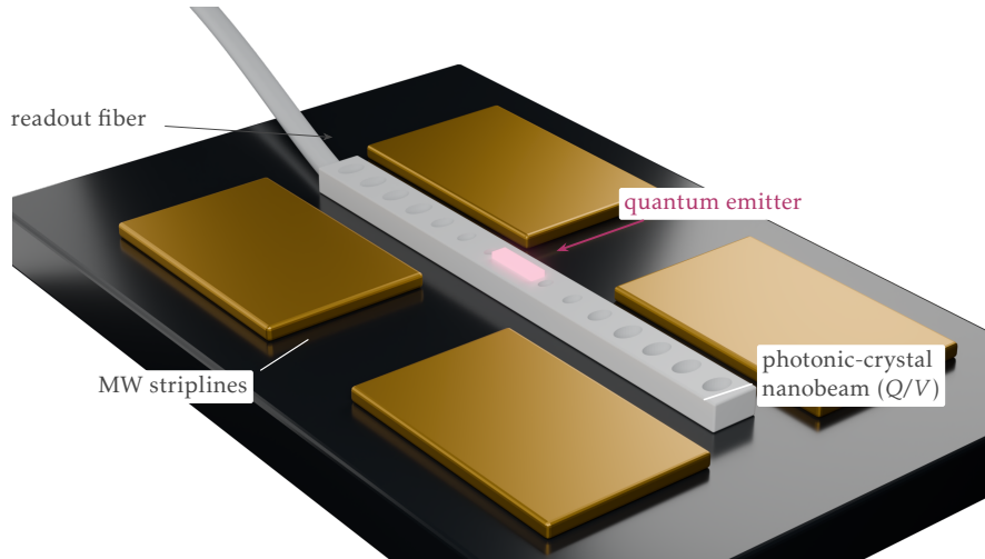
Figure 5: The kind of object this section is about: a quantum emitter inside a photonic-crystal nanobeam cavity, whose designed vacuum sets the coupling — and, through Eq. (3.1), the achievable F_Q . Microwave striplines drive the emitter’s spin; a fiber collects the photons.
