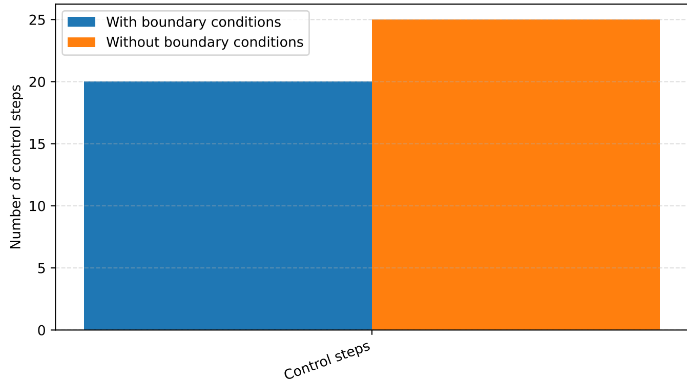
Control effort for LTI-MPC, N_p = 3 , 60-degree vessel
