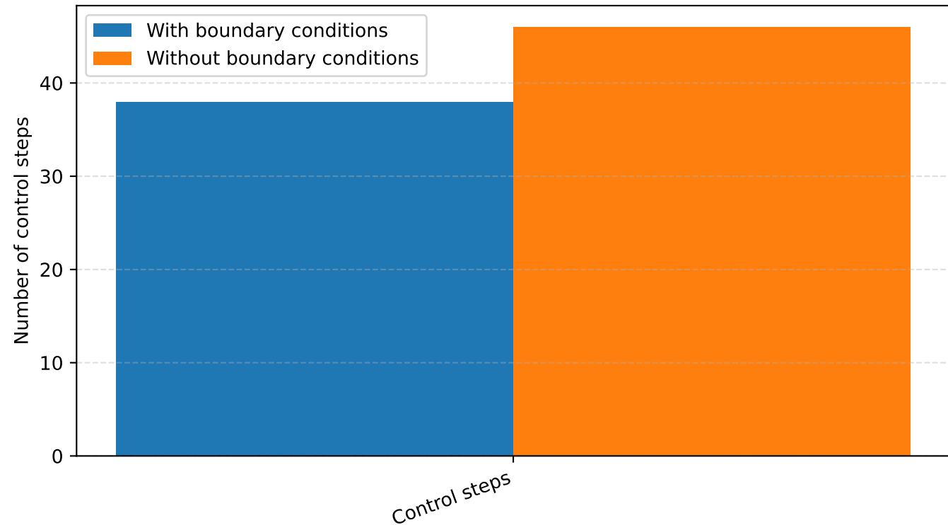
Control effort for LTI-MPC, N_p = 12 , 60-degree vessel
