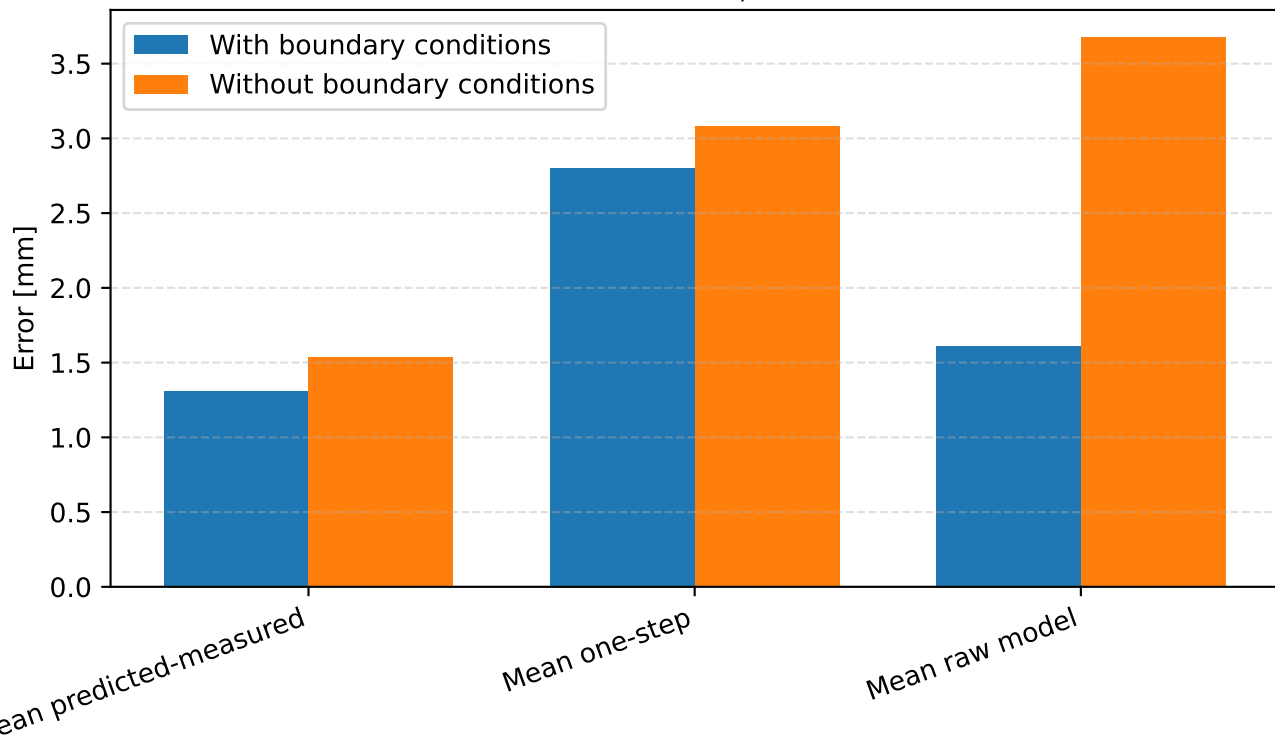
Prediction error for LTI-MPC, N_p = 12 , 60-degree vessel
