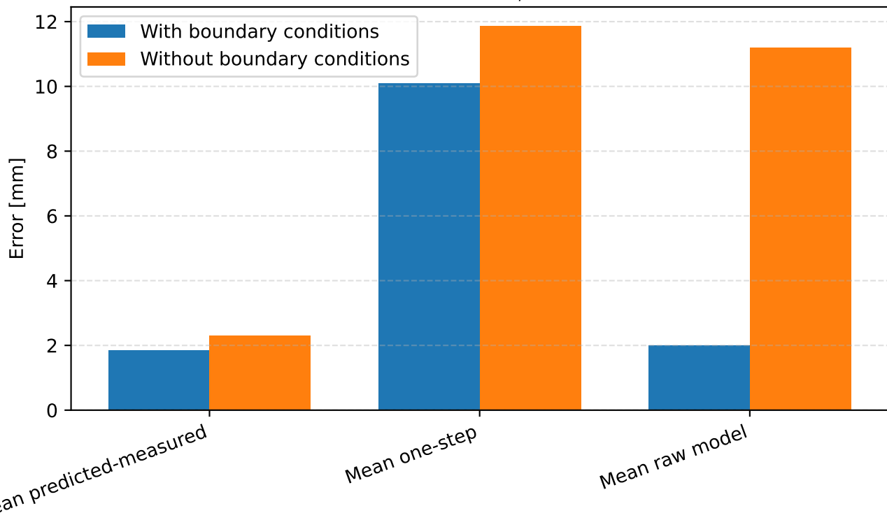
Prediction error for LTI-MPC, N_p = 3 , 60-degree vessel
