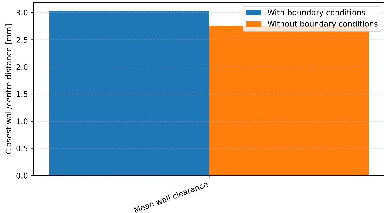
Wall clearance for LTI-MPC, N_p = 3 , 60-degree vessel
