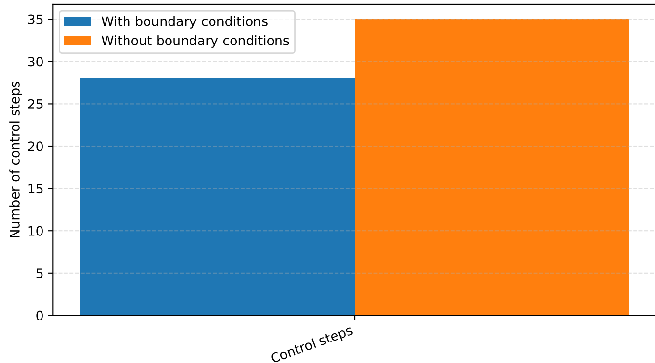
Control effort for LTI-MPC, N_p = 7 , 60-degree vessel
