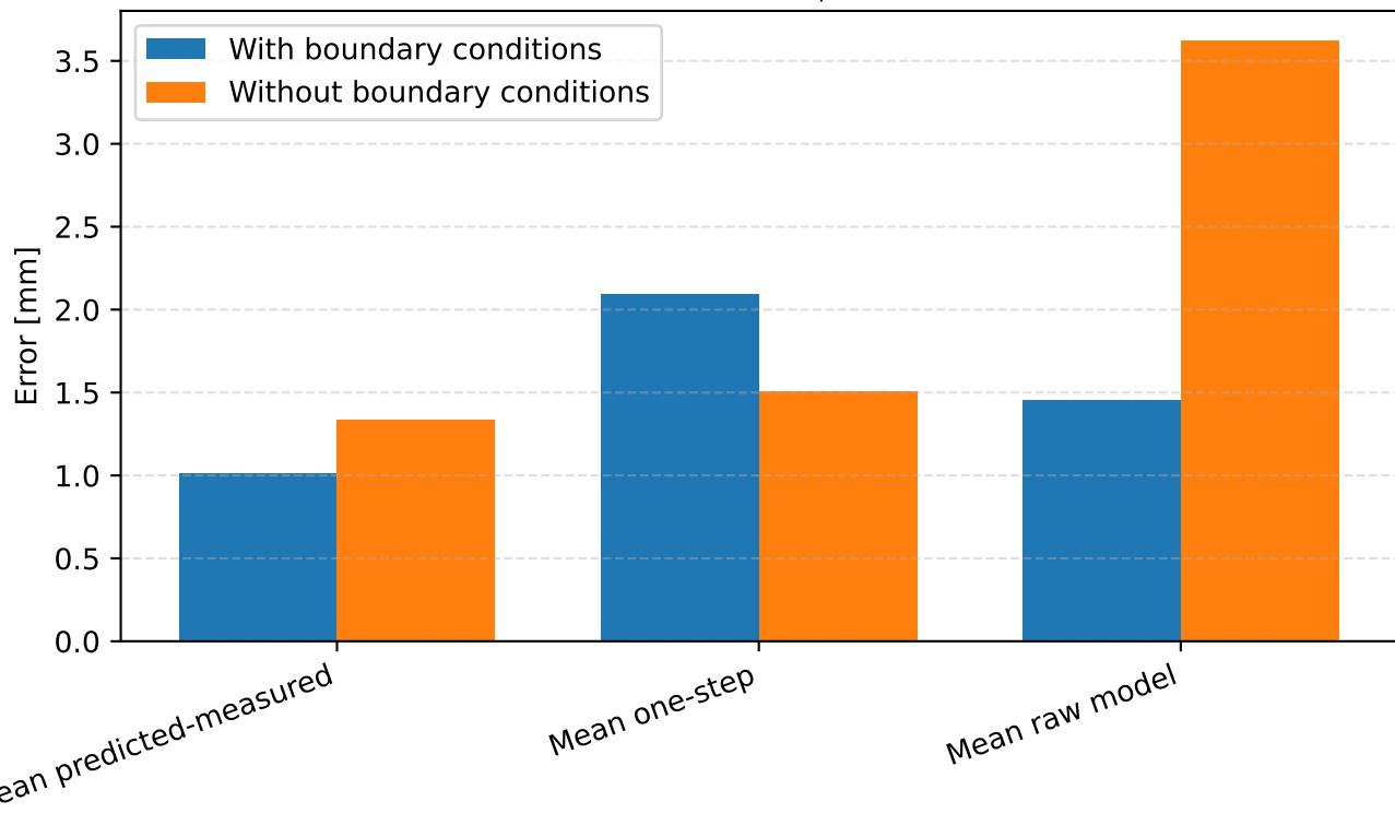
Prediction error for LTI-MPC, N_p = 7 , 60-degree vessel
