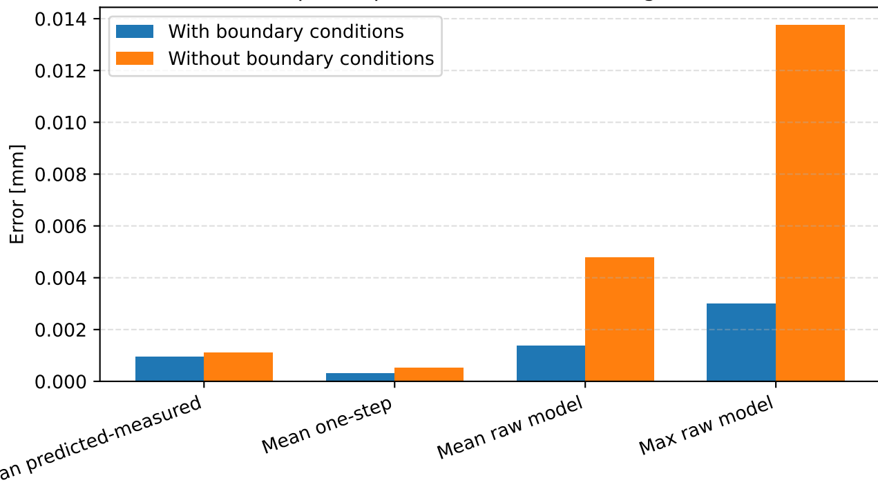
One-step MPC prediction error in 60-degree vessel
