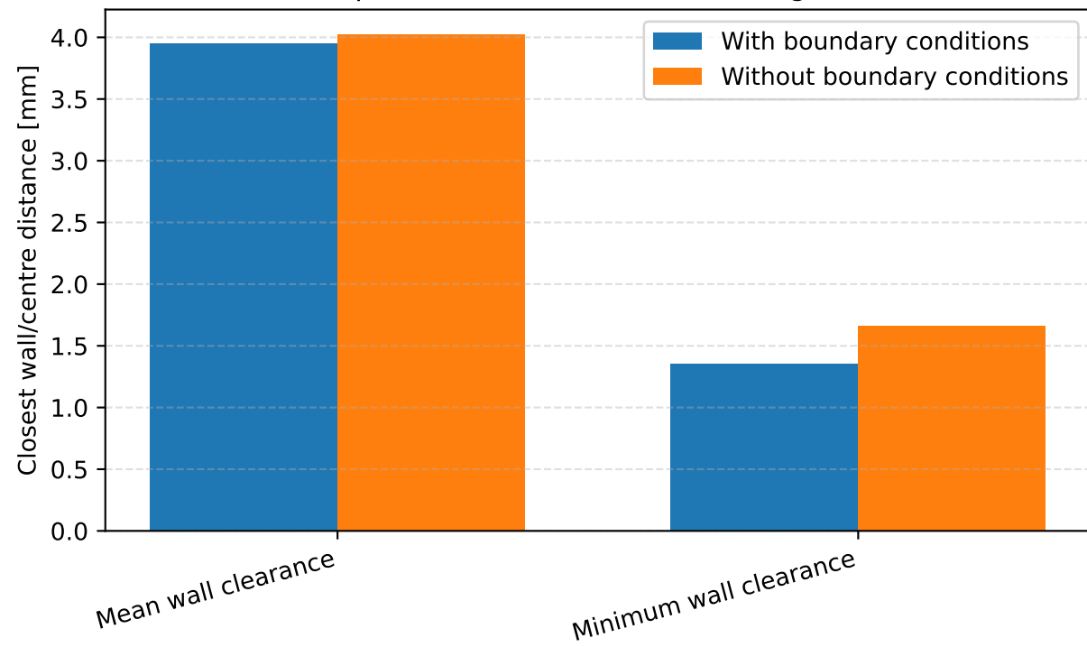
One-step MPC wall clearance in 60-degree vessel
