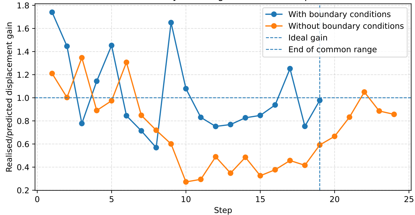
Realised Jacobian gain over MPC steps
