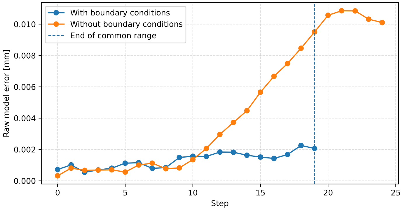
Raw model error over MPC steps
