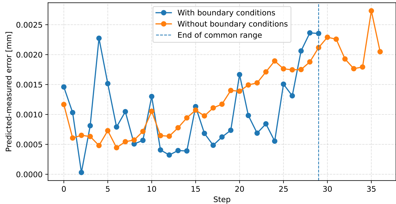
Predicted-measured error over MPC steps
