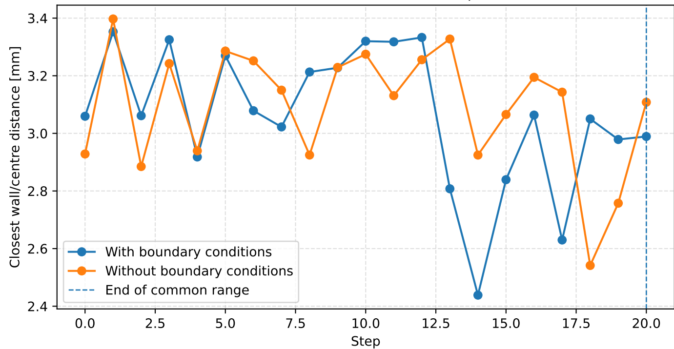
Wall clearance over MPC steps
