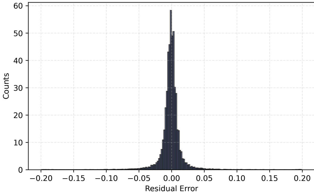
Residual Error Distribution (Zoomed)
