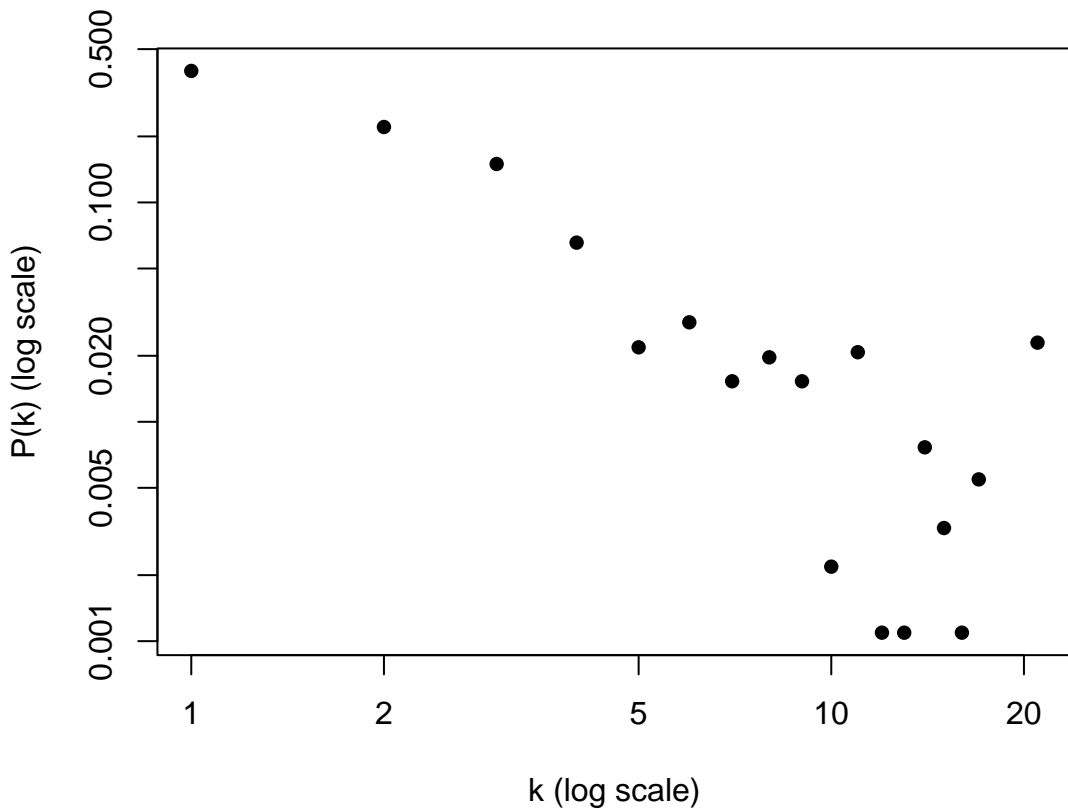
Degree distribution (log-log)
