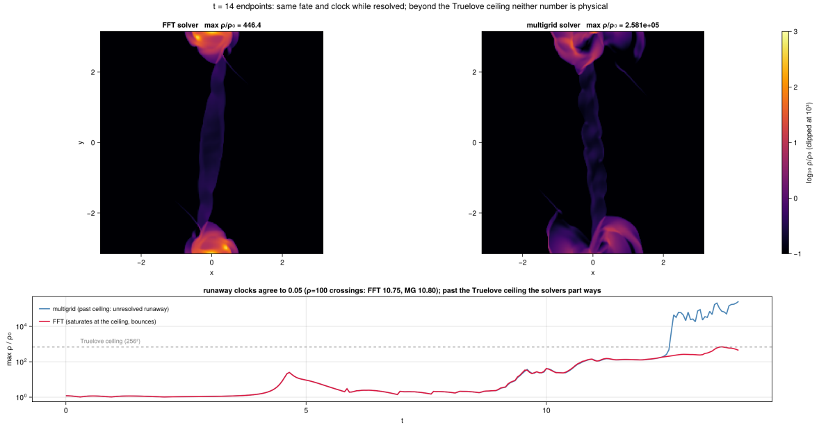
Figure 11: t = 14 endpoints of the 256^2 collapse under the two solvers: same fate (boundary knot wins, companion consumed) and runaway clocks agreeing to 0.05 ( p=100 crossings: FFT 10.75, MG 10.80); past the Truelove ceiling (dashed) the solvers diverge qualitatively — neither number is physical there.
