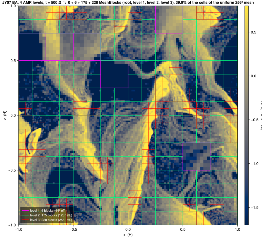
Figure 12: Run BA with four levels on 8^2 MeshBlocks at t = 500 (civdis, mesh drawn): magenta the six level-1 blocks ( 64^2 effective), spring green the 175 at level 2 ( 128^2 ) and red the 228 at the finest ( 256^2 , JY07's resolution), 40% of the cells of the uniform mesh. Rendered by validation/figures/plot_dust6_ba_amr3.jl with DUST6_BA=BA_amr4_mb8 .
