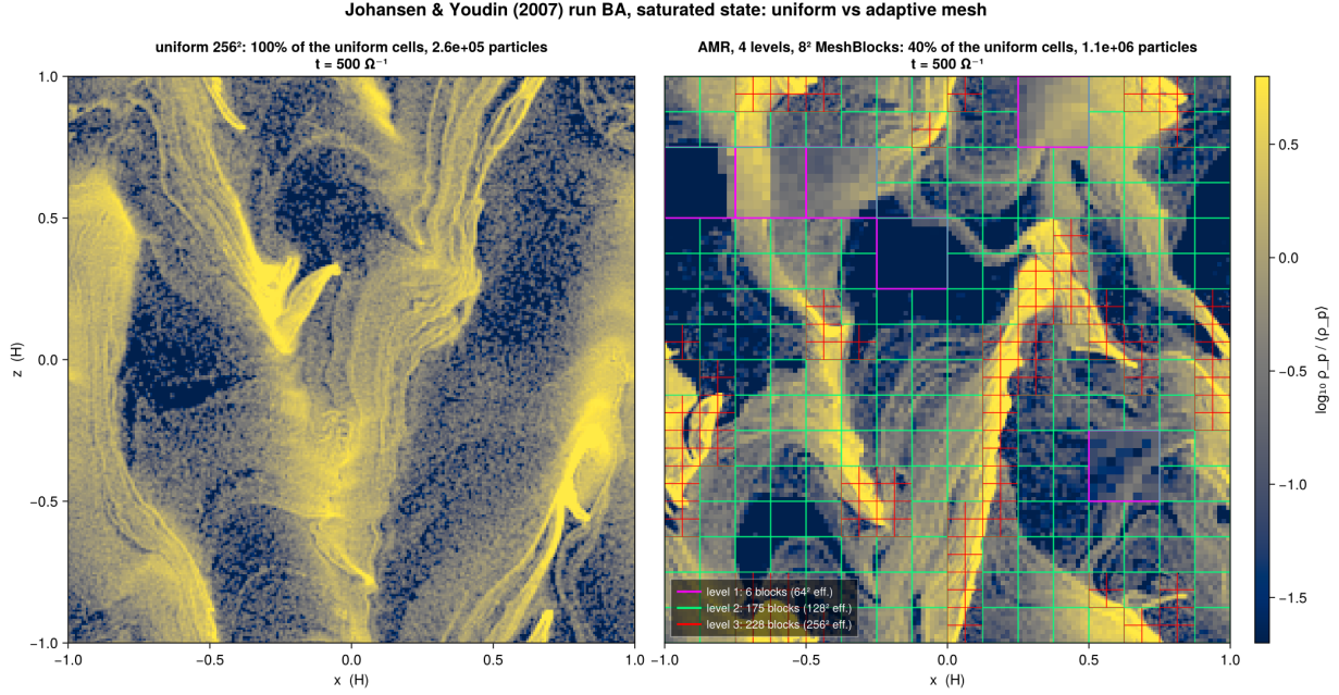
Figure 13: Run BA at t = 500 on the uniform 256^2 mesh (left, the Vista run) and on the four-level adaptive mesh with 8^2 MeshBlocks (right, mesh drawn), same colour scale. The particle counts in the titles are read from the histories at that time: the adaptive run's 1.1 \times 10^6 is the defect of §12.6, to be replaced by the repeat. Rendered by validation/figures/plot_dust6_ba_sbs.jl .
