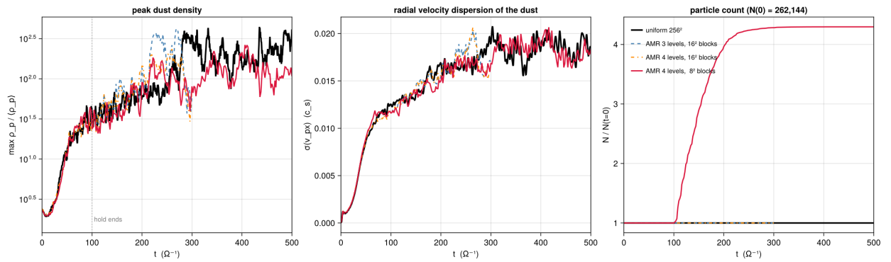
Figure 14: Run BA, the four meshes against time: the peak particle-mesh dust density, the radial velocity dispersion of the dust, and the particle count relative to the initial 262,144. The 16^2 -block runs hold their count through every re-refinement; the 8^2 -block run's rise from t = 100 is the uninitialised sampling level of §12.6. Rendered by validation/figures/plot_dust6_ba_hist.jl .
