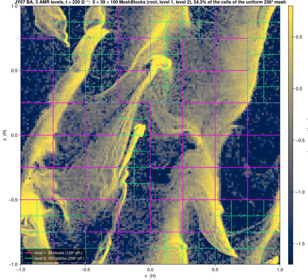
Figure 11: The same BA state at t = 230 with the mesh drawn (cividis): magenta outlines the 39 derefined level-1 MeshBlocks ( 128^2 effective) and spring green the 100 at the finest level ( 256^2 , JY07’s resolution), 54% of the cells of the uniform mesh. Every derefined block lies inside a void and the whole filament network is at the finest level; the speckle inside the coarse blocks is the particle shot noise of cells twice as wide at a tenth of the mean density. Rendered by validation/figures/plot_dust6_ba_amr3.jl .
