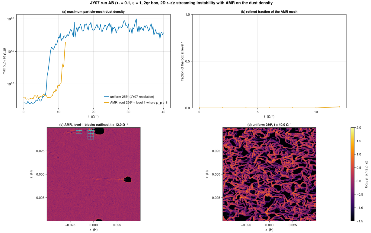
Figure 12: Phase 6: the JY07 run AB ( \tau_s = 0.1 , \epsilon = 1 , 2\eta r box, 2D r - z ) with AMR on the particle-mesh dust density (root 256^2 = \text{JY07's resolution} , one refined level above it, particles split on refinement) against the uniform 256^2 twin. (a) The maximum dust density. (b) The refined fraction of the box. (c) The AMR dust density at the finest resolution with the level-1 MeshBlocks outlined. (d) The uniform twin at the same time.
