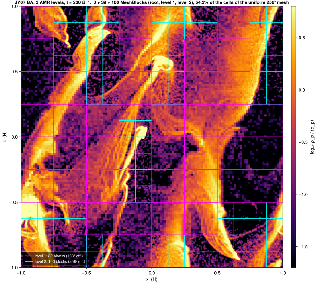
Figure 11: The same BA state at t = 230 with the mesh drawn: magenta outlines the 39 derefined level-1 MeshBlocks ( 128^2 effective) and cyan the 100 at the finest level ( 256^2 , JY07's resolution), 54% of the cells of the uniform mesh. Every derefined block lies inside a void and the whole filament network is at the finest level; the speckle inside the coarse blocks is the particle shot noise of cells twice as wide at a tenth of the mean density. Rendered by validation/figures/plot_dust6_ba_amr3.jl .
