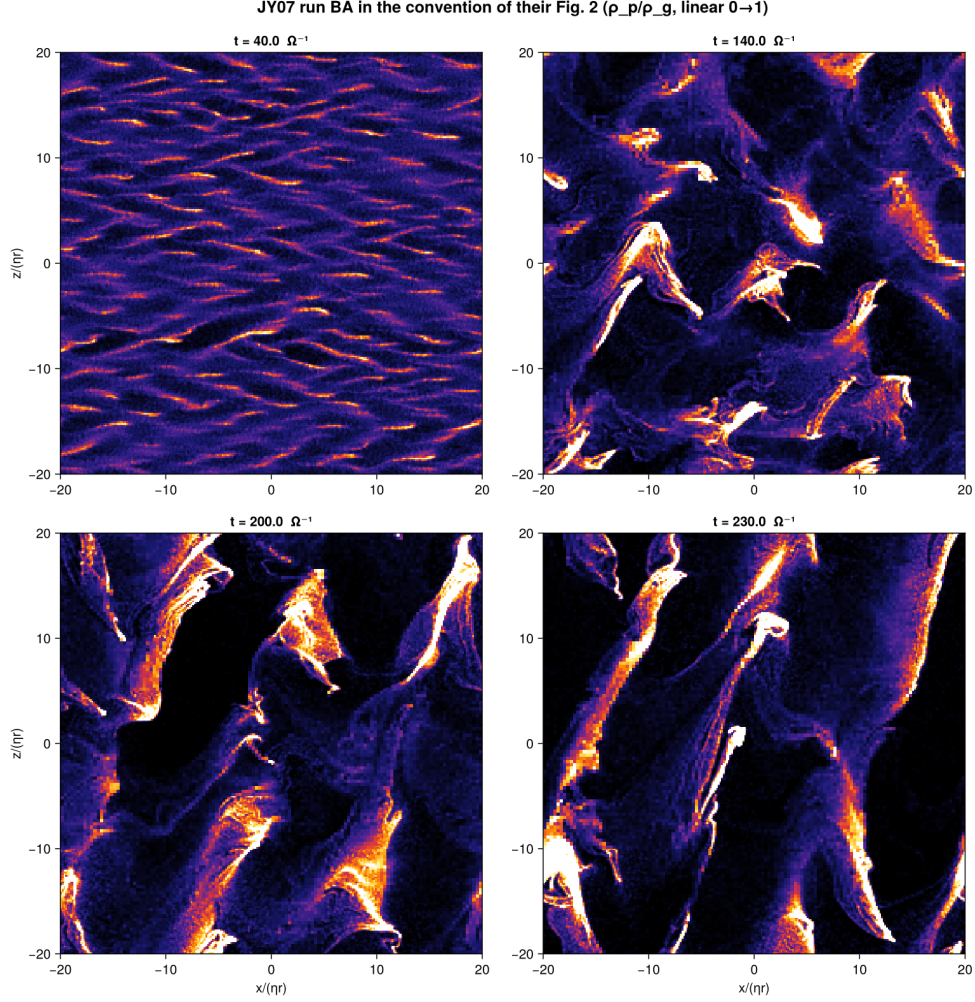
Figure 10: Run BA, three AMR levels, in the convention of JY07's Figure 2 ( \rho_p/\rho_g , linear 0 to 1, axes in \eta r ): the linear wave train at t = 40 , the cascade at t = 140 and 200, and the box-spanning, vertically aligned, radially tilted filament at t = 230 — their t = 40 , 80–120 and 160 frames respectively, about 70 \Omega^{-1} later.
