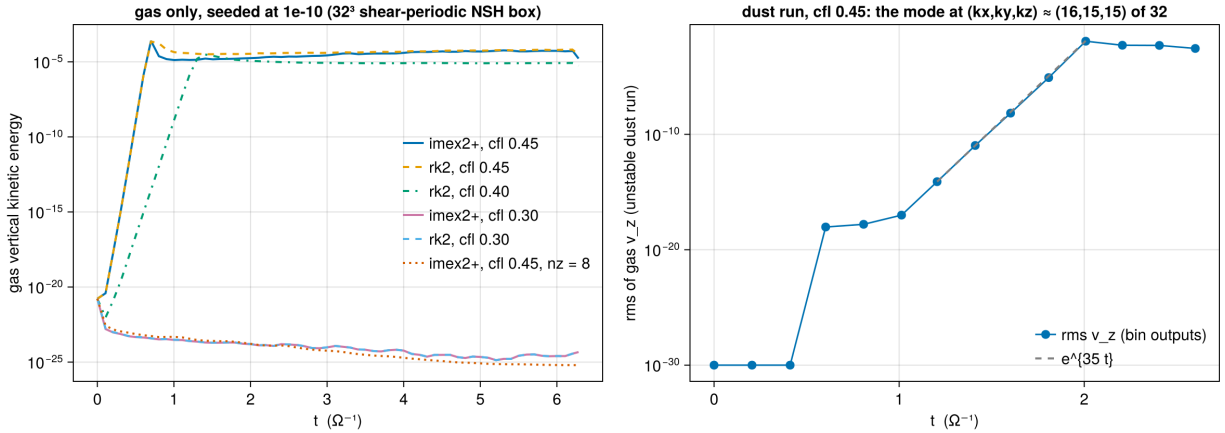
Figure 7: Phase 4d. Left: the gas-only 32^3 box seeded at 10^{-10} : the vertical kinetic energy grows at cfl \geq 0.4 under both integrators and decays at 0.3 and at n_z = 8 . Right: the rms gas v_z of the unstable dust run from its binary outputs, with the e^{35t} growth of the checkerboard mode.
