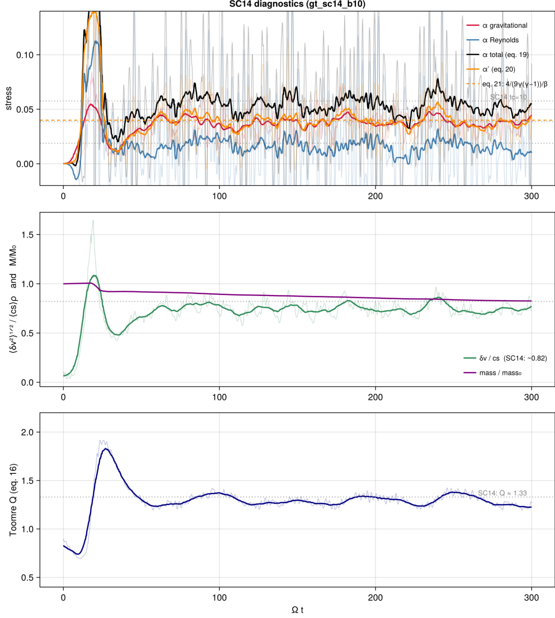
Figure 5: The full-size SC14 \beta = 10 run in their Figure-2 form (thick: 12\Omega^{-1} boxcar; dotted: SC14's t_c=10 values; dashed: their eq.-21 energy-balance line): stresses, \delta v/c_s and mass, Toomre Q .
