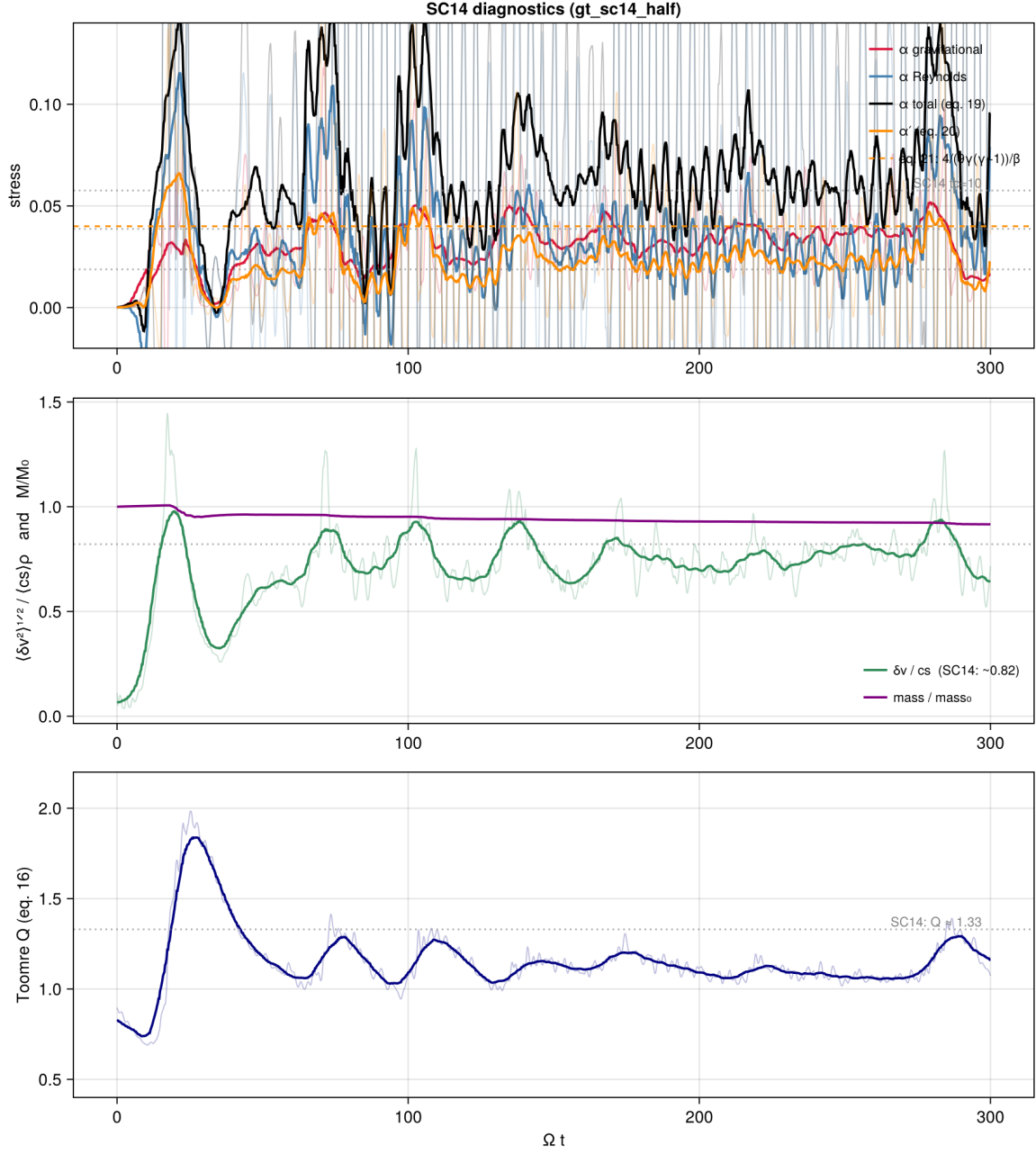
Figure 12: The half-box \beta = 10 run in SC14's Figure-2 form (thin: raw history; thick: 12\Omega^{-1} boxcar as in the paper; dotted gray: their tc=10 values; dashed: the eq.-21 energy-balance line). Top: stresses (gravitational, Reynolds, total, \alpha' ); middle: \delta v/c_s and M/M_0 ; bottom: Toomre Q . The quasi-periodic box-scale bursts are the half-width signature discussed in the text.
