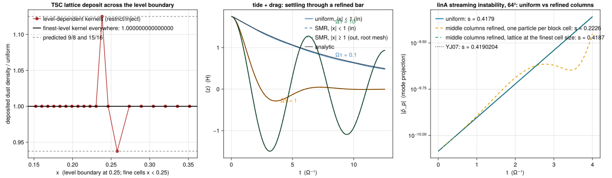
Figure 7: Phase 5. Left: the deposited dust density across the x_1 level boundary of the SMR NSH lattice at t = 0 , restrict/inject scheme (the predicted 9/8 and 15/16 ) and finest-level deposits (exactly 1). Middle: \langle z \rangle(t) of the settling test particles, uniform mesh and SMR twin, the population that crosses into the refined bar and the one that stays on the root mesh, against the analytic damped oscillator. Right: the linA mode amplitude on the uniform 64^2 mesh and with the two middle radial columns refined.
