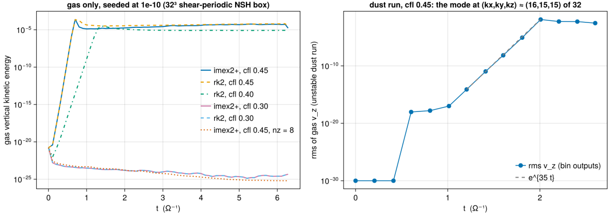
Figure 8: Phase 4d. Left: the gas-only 32^3 box seeded at 10^{-10} : the vertical kinetic energy grows at cfl \geq 0.4 under both integrators and decays at 0.3 and at n_z = 8 . Right: the rms gas v_z of the unstable dust run from its binary outputs, with the e^{35t} growth of the checkerboard mode.
