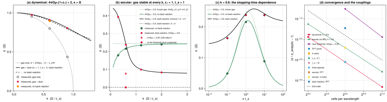
Figure 7: The rotating dusty Jeans problem with superparticle dust. (a) The dynamical regime: Chandrasekhar’s gas-only relation and the gas + dust curve with and without back-reaction, with the measured rates. (b) The secular regime, gas stable at every k : back-reaction off, the one-way-drag mode against the k -independent frozen-gas rate; back-reaction on, growth only because the mixture exceeds \kappa^2 ( 4\pi G = 0.6 ), and the neutral point at the threshold. (c) The same against the stopping time at k = 0.6 . (d) Convergence and the couplings.
