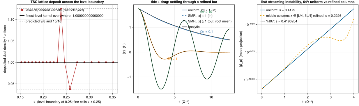
Figure 7: Phase 5. Left: the deposited dust density across the x_1 level boundary of the SMR NSH lattice at t = 0 , restrict/inject scheme (the predicted 9/8 and 15/16) and finest-level deposits (exactly 1). Middle: \langle z \rangle(t) of the settling test particles, uniform mesh and SMR twin, the population that crosses into the refined bar and the one that stays on the root mesh, against the analytic damped oscillator. Right: the linA mode amplitude on the uniform 64^2 mesh and with the two middle radial columns refined.
