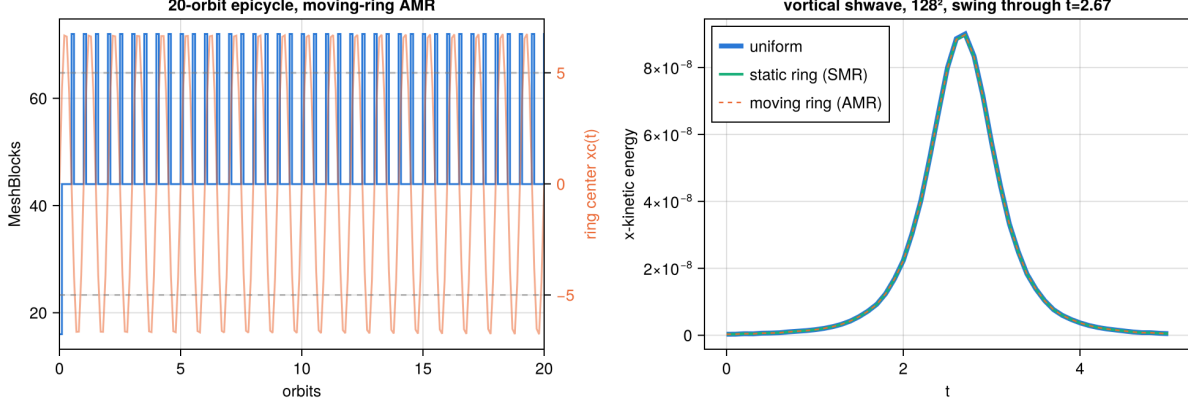
Figure 3: Phase 0c. Left: MeshBlock count (blue, left axis) in the 20-orbit moving-ring epicycle AMR run, with the prescribed ring center x_c(t) = 7 \sin t (orange, right axis; dashed lines mark the vetoed boundary columns beyond |x_1| = 5 ). Rings are destroyed near every turning point and re-created on the way back, 2296 blocks created / 2240 destroyed in total. Right: x -KE history of the 128^2 vortical shwave through the swing — uniform, static SMR ring, and moving-ring AMR are visually indistinguishable (moving vs. static ring: 1.8 \times 10^{-4} of peak).
