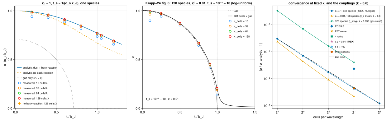
Figure 6: The dusty Jeans instability with superparticle dust. Left: \epsilon_0 = 1 , t_s = 1/(c_s k_J) — the eigenproblem with and without back-reaction, the gas-only curve, and the gas-mode rates measured at 16 to 128 cells per wavelength. Middle: the replica of Krapp et al. (2024) Fig. 6 — 128 species, \epsilon_0 = 0.01 , t_s log-uniform in [10^{-4}, 10] , \sigma in their units — at their six wavenumbers and four resolutions; the dotted line is the dust-free cutoff. Right: convergence at fixed k (the strong-dust case, the linear 128-species mixture, and the replica’s cutoff mode) with the other couplings and solvers at k/k_J = 0.6 .
