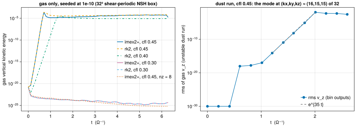
Figure 7: Phase 4d. Left: the gas-only 32^3 box seeded at 10^{-10} : the vertical kinetic energy grows at \text{cfl} \geq 0.4 under both integrators and decays at 0.3 and at n_z = 8 . Right: the rms gas v_z of the unstable dust run from its binary outputs, with the e^{35t} growth of the checkerboard mode.
