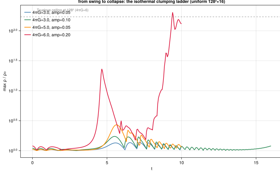
Figure 7: Maximum density vs. time for the nonlinear ladder: two bounces, a marginal miss, and the collapse, with the 128^2 Truelove ceiling marked.
