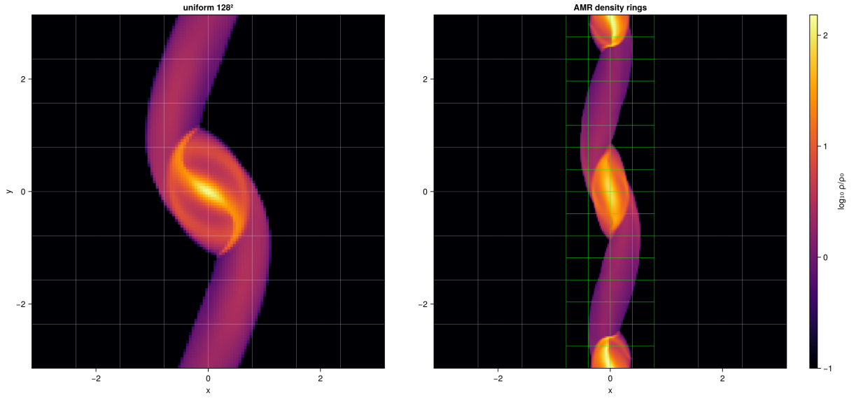
Figure 9: Final ( t = 10 ) density of the collapse runs, \log_{10} \rho / \rho_0 at the z mid-plane, with the MeshBlock structure drawn (green = level 1): uniform 128^2 vs. the density-triggered AMR rings. The level-1 ring has contracted onto the clump's x_1 columns — the annular-policy answer to zooming under FARGO.
