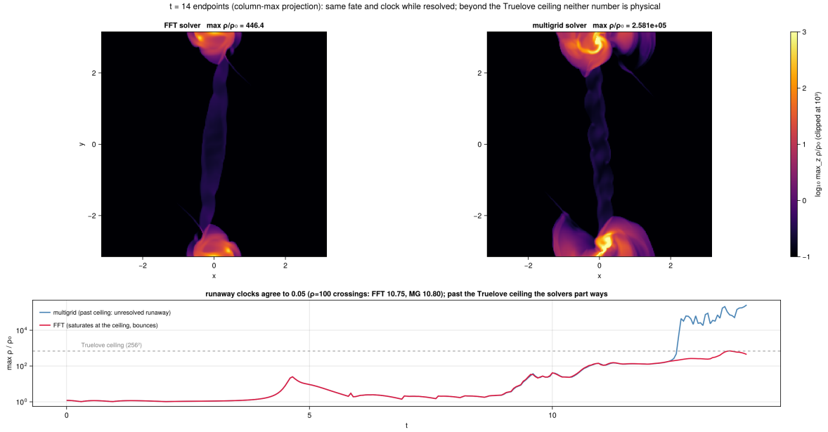
Figure 11: t = 14 endpoints of the 256^2 collapse under the two solvers: same fate (boundary knot wins, companion consumed) and runaway clocks agreeing to 0.05 while resolved; beyond the Truelove ceiling (dashed) the solvers diverge qualitatively — neither number is physical there.
