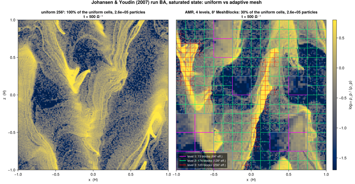
Figure 13: Run BA at t = 500 on the uniform 256^2 mesh (left, the Vista run) and on the four-level adaptive mesh with 8^2 MeshBlocks (right, mesh drawn; the repeat on the fixed binary), same colour scale. The particle counts in the titles are read from the histories at that time: 262,144 on both sides. Rendered by validation/figures/plot_dust6_ba_sbs.jl .
