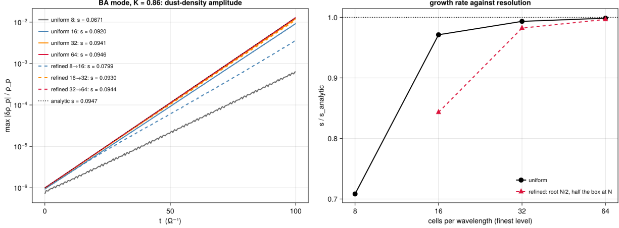
Figure 16: The BA-parameter linear mode ( K_x = K_z = 0.86 , s = 0.09472 ): the peak dust-density amplitude against time on uniform meshes of 8–64 cells per wavelength (solid) and on refined meshes with the root at half that and the middle half of the box refined once (dashed), the analytic growth dotted; and the measured rate over the analytic one against the cells per wavelength at the finest level. Rendered by validation/figures/plot_dust6_lin_ba.jl .
