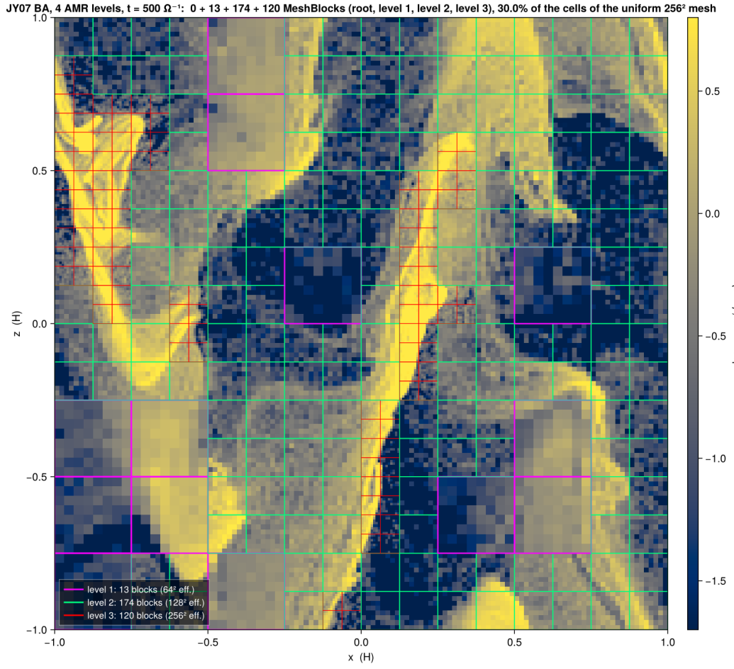
Figure 12: Run BA with four levels on 8^2 MeshBlocks at t = 500 , the repeat on the fixed binary (civdis, mesh drawn): magenta the 13 level-1 blocks ( 64^2 effective), spring green the 174 at level 2 ( 128^2 ) and red the 120 at the finest ( 256^2 , JY07's resolution), 30% of the cells of the uniform mesh. Rendered by validation/figures/plot_dust6_ba_amr3.jl with DUST6_BA=BA_amr4_mb8_fix .
