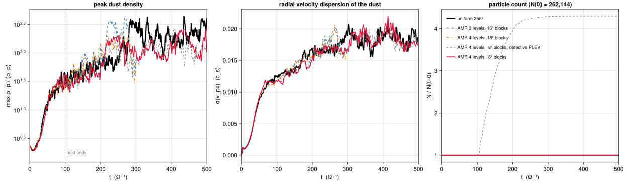
Figure 14: Run BA, the four meshes against time: the peak particle-mesh dust density, the radial velocity dispersion of the dust, and the particle count relative to the initial 262,144. The 16^2 -block runs and the repeat of the 8^2 -block run (crimson) hold their count through every re-refinement; the grey dashed rise from t = 100 is the original 8^2 -block run with the uninitialised sampling level of §12.6. Rendered by validation/figures/plot_dust6_ba_hist.jl .
