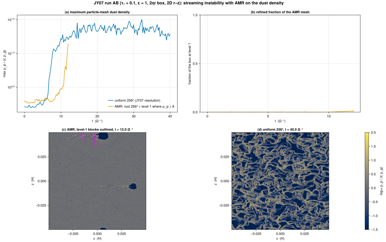
Figure 15: Phase 6: the JY07 run AB ( \tau_s = 0.1 , \epsilon = 1 , 2\eta r box, 2D r - z ) with AMR on the particle-mesh dust density (root 256^2 = \text{JY07's resolution} , one refined level above it, particles split on refinement) against the uniform 256^2 twin. (a) The maximum dust density. (b) The refined fraction of the box. (c) The AMR dust density at the finest resolution with the level-1 MeshBlocks outlined. (d) The uniform twin at the same time.
