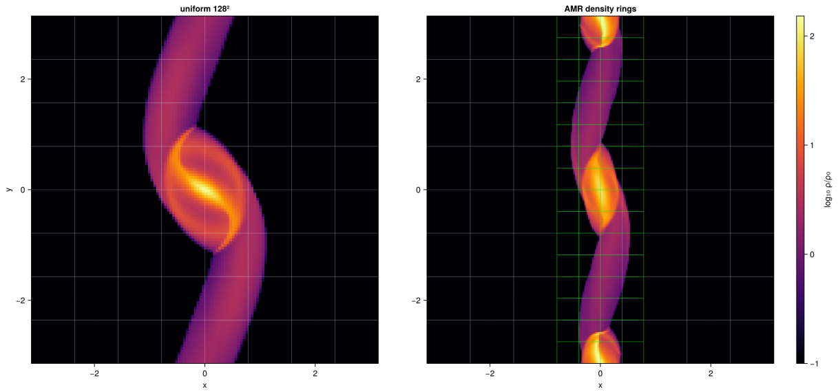
Figure 12: Final ( t = 10 ) density of the collapse runs, \log_{10} \rho/\rho_0 at the z mid-plane, with the MeshBlock structure drawn (green = level 1): uniform 128^2 vs. the density-triggered AMR rings. The level-1 ring has contracted onto the clump's x_1 columns — the annular-policy answer to zooming under FARGO.
