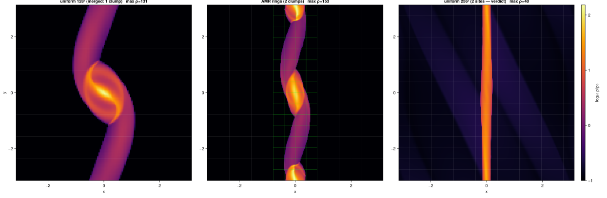
Figure 11: The two-clump discriminator: final ( t = 10 ) \log_{10} \rho for uniform 128^2 (one merged clump), the AMR run (two clumps, level-1 outlines), and uniform 256^2 — which reproduces the AMR run’s two-site structure at matched resolution.
