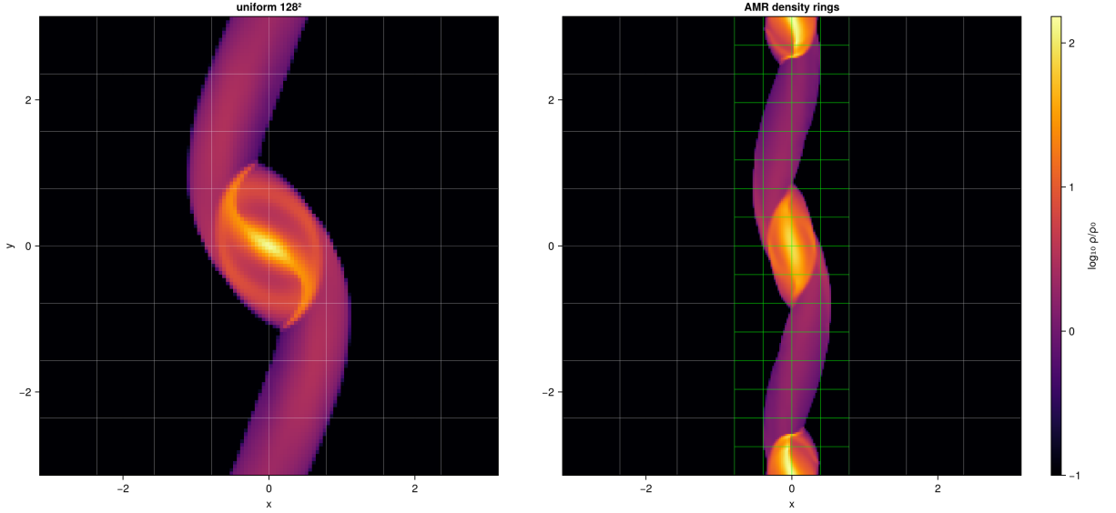
Figure 12: Final ( t = 10 ) density of the collapse runs, \log_{10} \rho/\rho_0 at the z mid-plane, with the MeshBlock structure drawn (green = level 1): uniform 128^2 vs. the density-triggered AMR rings. The level-1 ring has contracted onto the clump’s x_1 columns — the annular-policy answer to zooming under FARGO.
