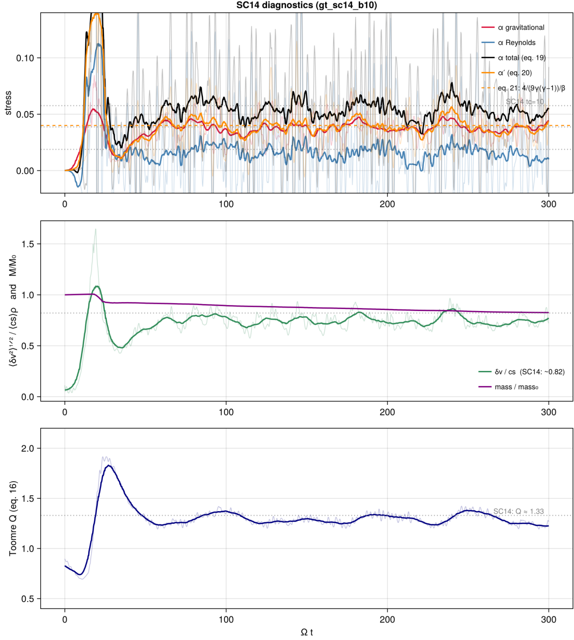
Figure 12: The full-width ( 64H ) \beta = 10 run in SC14's Figure-2 form (thin: raw history; thick: 12\Omega^{-1} boxcar as in the paper; dotted gray: their tc=10 values; dashed: the eq.-21 energy-balance line). Top: stresses (gravitational, Reynolds, total, \alpha' ); middle: \delta v/c_s and M/M_0 ; bottom: Toomre Q .
