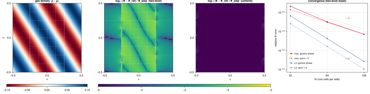
Figure 4: The static shwawe test at the generic shear phase ( 64^3 root, level-1 ring over |x| < 1/4 , block outlines in white). First panel: the sheared density mode. Second: \log_{10} relative potential error against the root-grid closed form (eq. 10) on the two-level mesh — the error lives in the fine region (root–fine eigenvalue mismatch, the 6 \times 10^{-4} plateau of §7.4), peaks in the first fine-cell layer on the refinement interfaces (dashed; bright cells modulated by the mode phase, pinched at its zero-crossing curves), and shows no feature at the shear-periodic faces x = \pm 1/2 . Third: the same metric on the uniform Phase-1 run — pure remap truncation at 5 \times 10^{-6} , three decades below the interface and eigenvalue structure. Fourth: error vs. resolution at both shear phases — L_2 second order, interface peak first order, the two phases nearly coincident.
