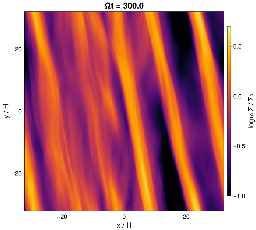
Figure 15: Vertically integrated surface density \log_{10} \Sigma / \Sigma_0 of the full-width box at \Omega t = 300 : the trailing gravito-turbulent wake field, with \Sigma contrasts of \sim \times 5 .
