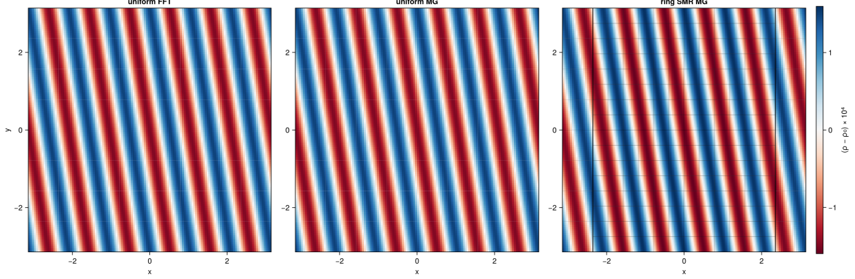
Figure 6: Final ( t = 8 = 2t_{\text{swing}} ) density deviation (\rho - \rho_0) \times 10^4 at the z mid-plane for the three swing runs: uniform FFT, uniform multigrid, and the level-1 interior-ring SMR run (block outlines drawn; the heavier lines mark the refinement-level boundary). The two uniform panels are indistinguishable ( \leq 2 \times 10^{-7} everywhere); the SMR panel carries the same trailing wave with the amplitude difference of §7.5.
