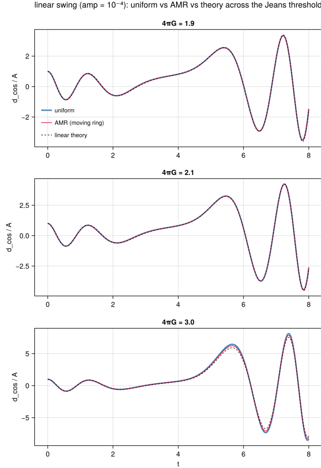
Figure 7: The linear swing grid: uniform (blue) vs. moving-ring AMR (red) vs. the linearized ODE (dashed) at 4\pi G = 1.9, 2.1, 3.0 , all at amp = 10^{-4} .
