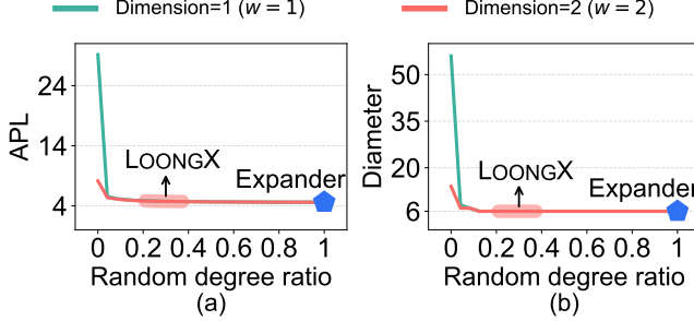
Figure 3: (a) APL and (b) diameter under varying random degree ratios at 10k-nodes.
