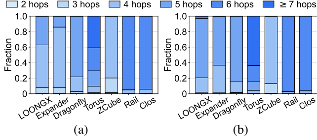
Figure 22: Hop-count distribution for GPU-to-GPU paths at different cluster scales: (a) 2.5k and (b) 10k nodes.
