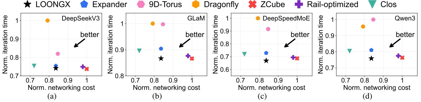
Figure 11: Iteration time vs. networking cost for concurrent workloads in a 10k-nodes multi-tenant AI cluster: (a) DeepSeekV3, (b) GLaM, (c) DeepSpeedMoE, and (d) Qwen3.
