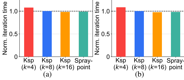
Figure 16: Iteration time under different routing for (a) 1k-nodes and (b) 10k-nodes.
