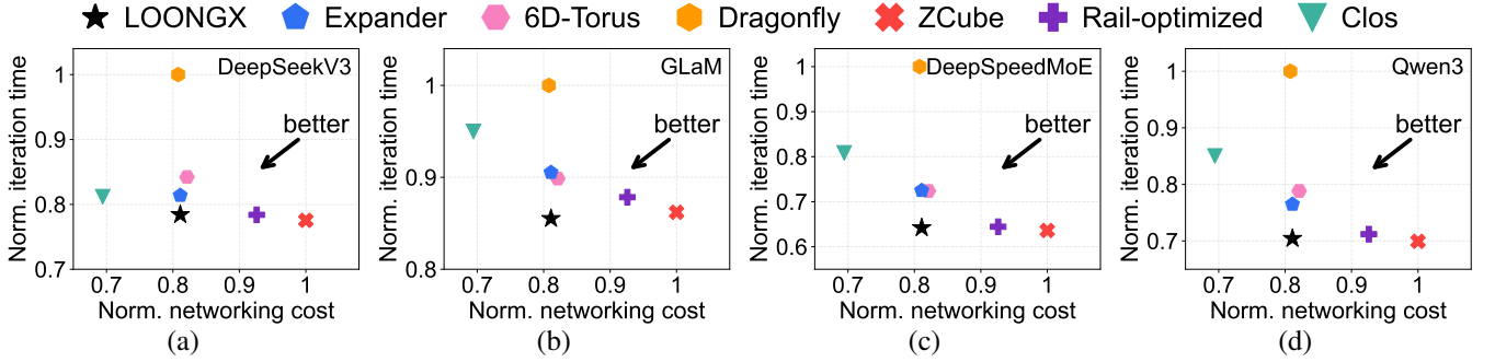
Figure 10: Iteration time vs. networking cost for concurrent workloads in a 2.5k-nodes multi-tenant AI cluster: (a) DeepSeekV3, (b) GLaM, (c) DeepSpeedMoE, and (d) Qwen3.
