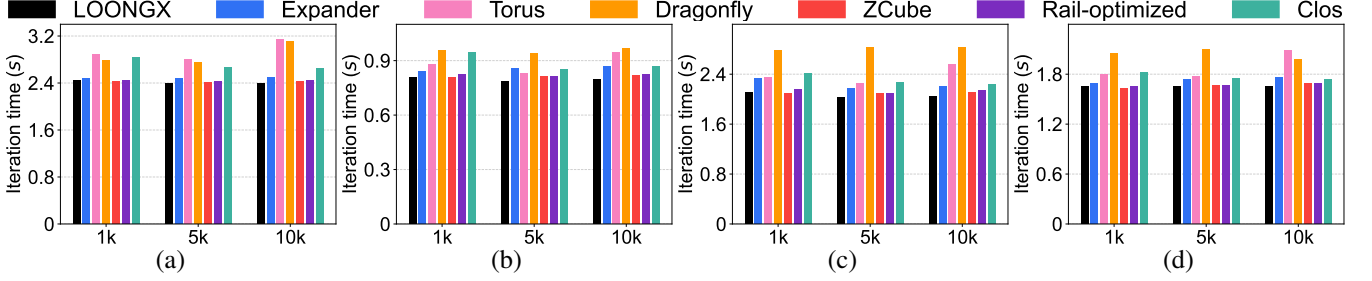
Figure 9: Iteration time across different AI cluster scales under isolated training workloads: (a) DeepSeekV3, (b) GLaM, (c) DeepSpeedMoE, and (d) Qwen3.
