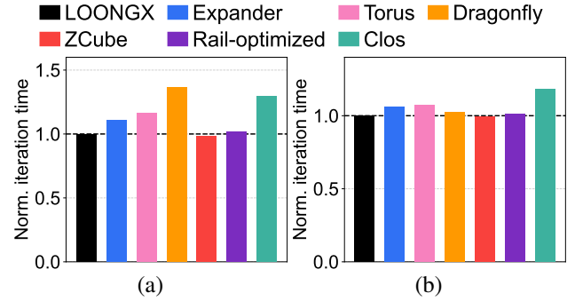
Figure 19: Normalized iteration time under (a) topology-aware and (b) random placement.
