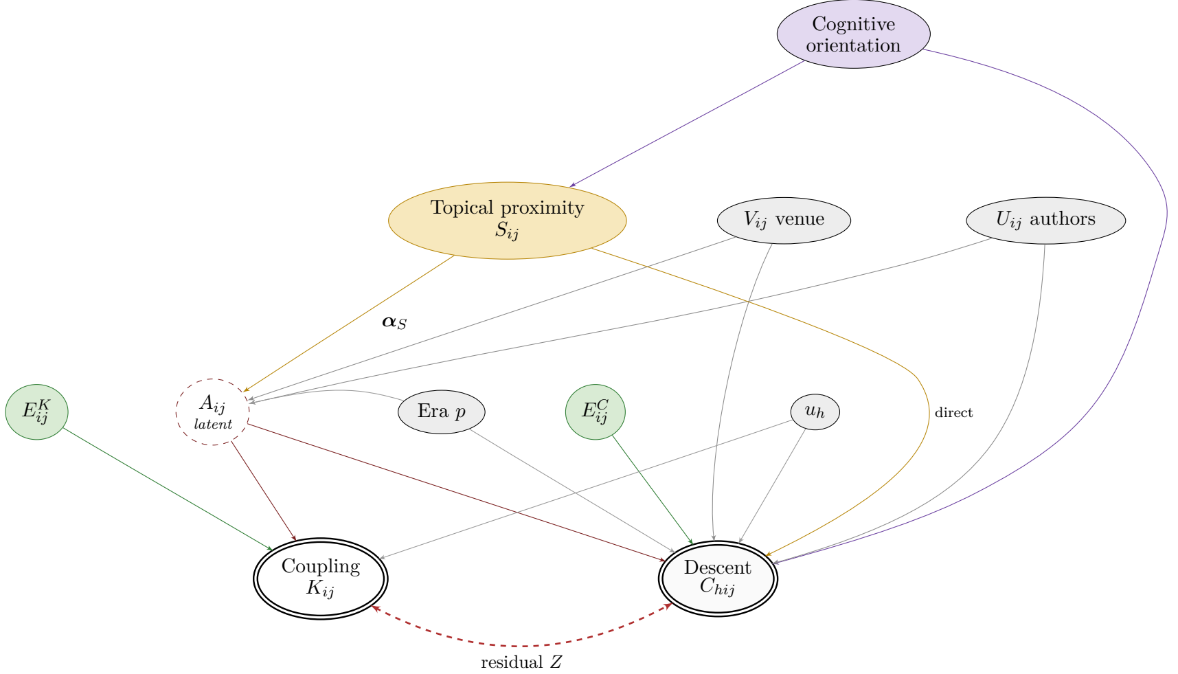
Figure 1: The conceptual model. Topical proximity S_{ij} shapes a shared knowledge base A_{ij} , which we cannot observe (dashed). Coupling K_{ij} and descent C_{hij} are two observed manifestations of it (double outlines). Remaining arrows are the alternative reasons a connection might form: shared authors U_{ij} , shared venues V_{ij} , opportunity E^K and E^C , individual work salience u_h , and era p . Drawn in Pearl’s semi-Markovian notation; the dashed double-headed arc marks common causes of both indicators that we cannot measure, such as reciprocal reviewing obligations and shared institutional context.
