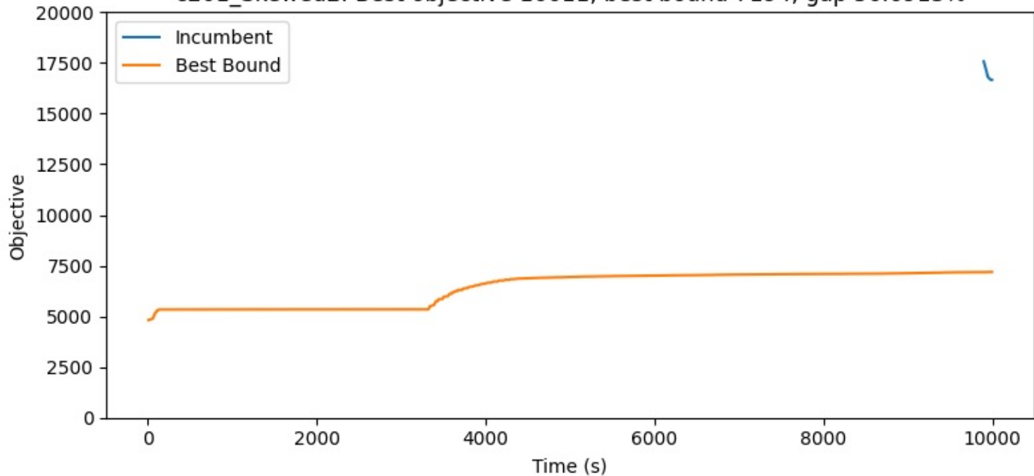
c201_Skewed2: Best objective 16611, best bound 7194, gap 56.6913%
