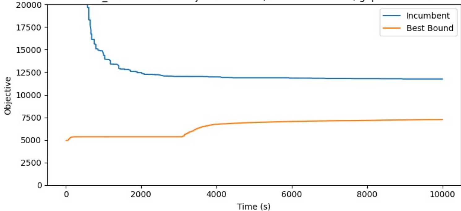
c201_Skewed1: Best objective 11752, best bound 7260, gap 38.2233%
