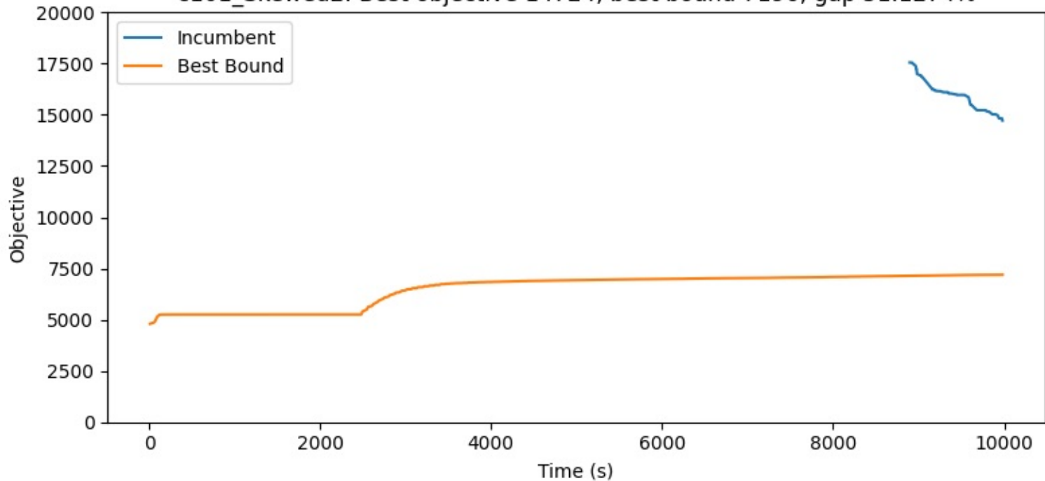
c101_Skewed2: Best objective 14724, best bound 7196, gap 51.1274%
