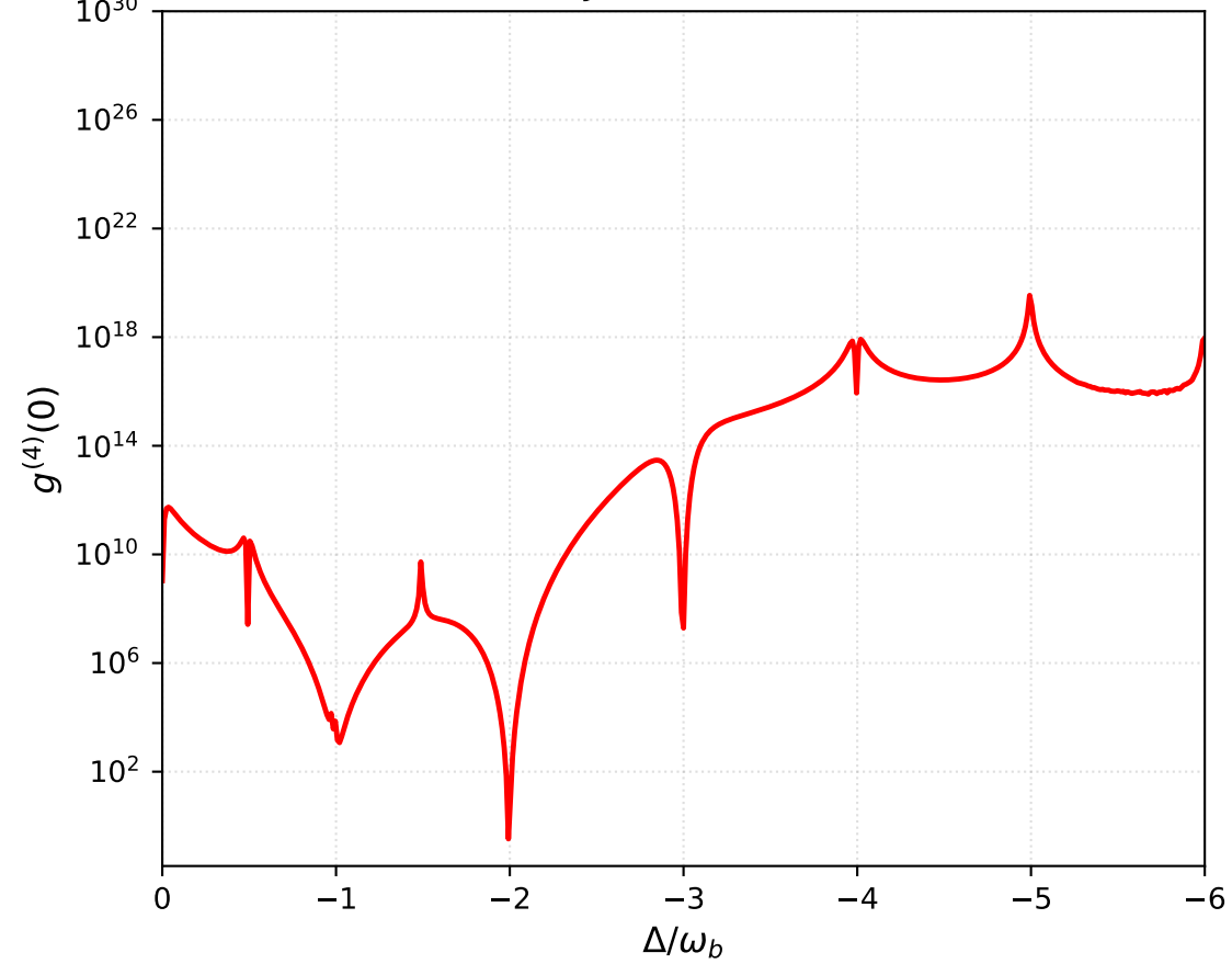
J/\omega b = 1.0
